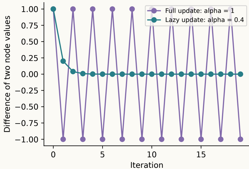
Periodicity without laziness
