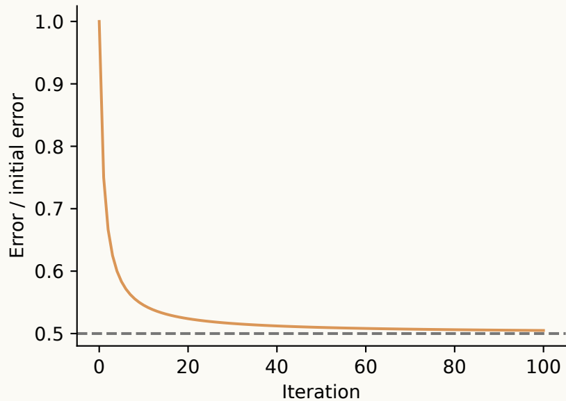
Every step has a home edge; error persists
