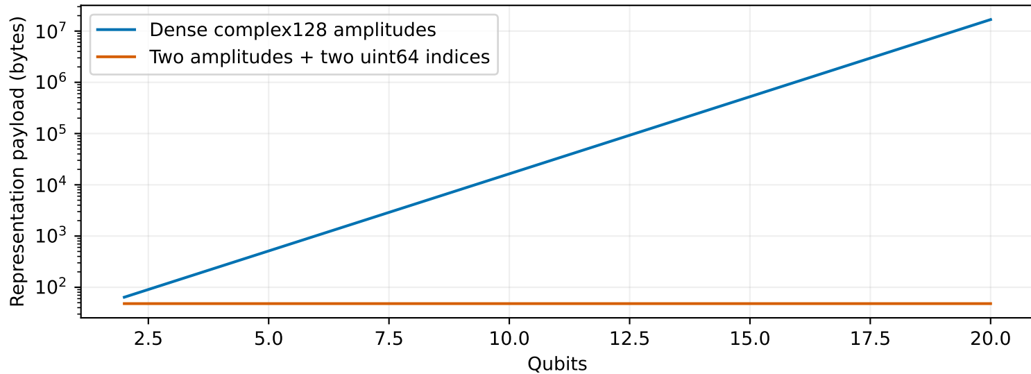
Same GHZ state, different classical representations
