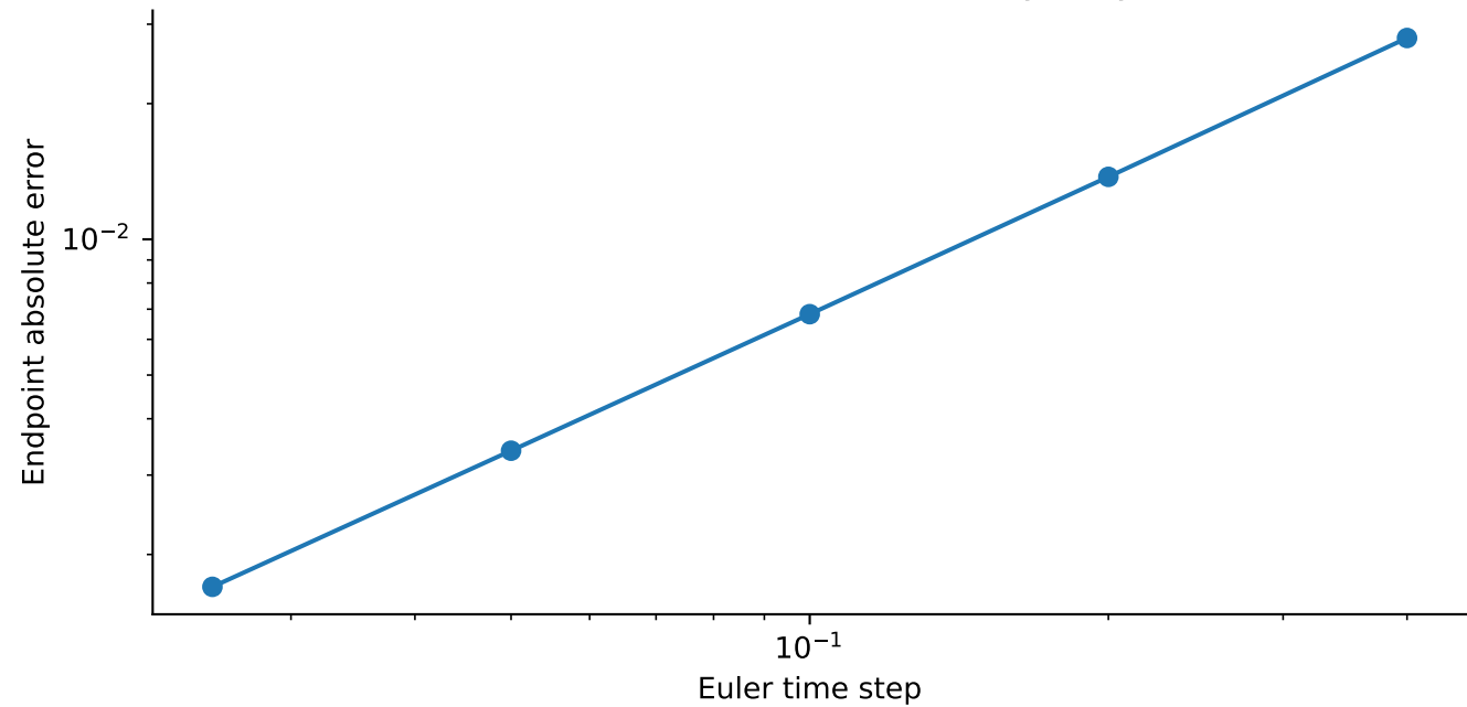
Discretization error in a known analytic system
