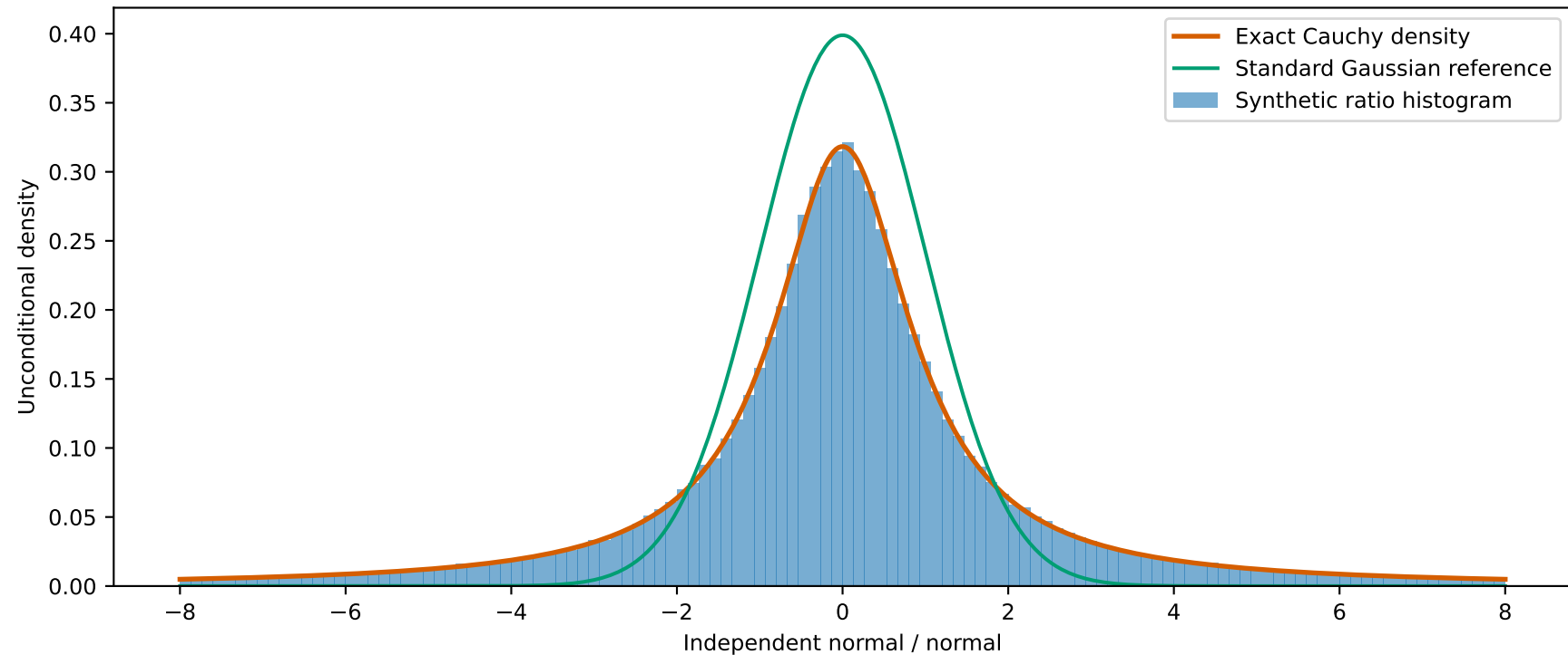
A projective ratio can be heavy-tailed without a heavy-tailed source
