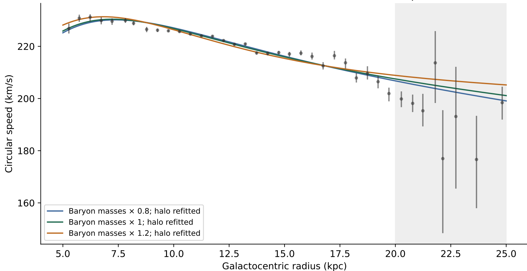
Similar rotation curves can have different mass decompositions
