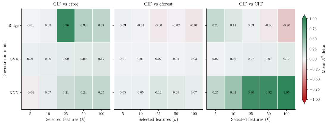
Figure 7: Regression CIF margins against ctrees, cforest, and CIT by downstream learner and value of k . Each plotted value is the mean R^2 difference, CIF minus comparator, for one downstream learner and one value of k ; positive values favor CIF. Dataset counts by k are 8, 8, 7, 7, and 6 for each comparison. Large positive plotted values can reflect negative mean R^2 for the comparator. Numeric labels show the unclipped values; the color scale is clipped at \pm 1 for readability. Values are means over datasets; the bootstrap intervals for the pooled differences are in ??.
