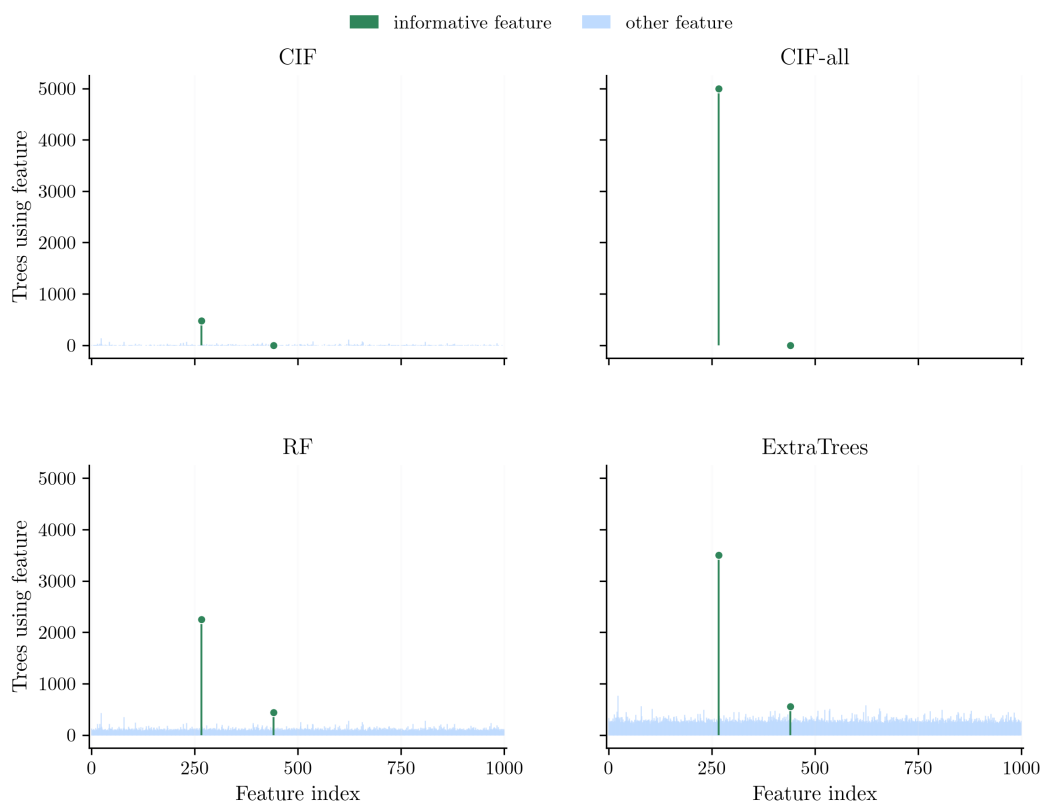
Figure 5: Tree-level feature use in one sparse classification forest design ( n = 250 , p = 1,000 , two informative features). Counts are the number of trees using each feature in at least one split, pooled over five fits of 1,000 trees each, so the shared vertical axis runs to 5,000. CIF samples a subset of features at each node; CIF-all evaluates all nonconstant features.
