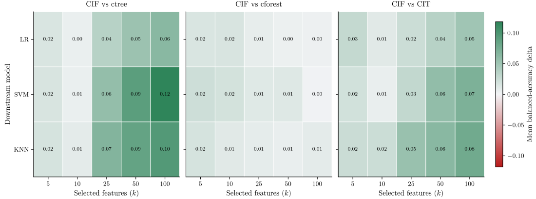
Figure 6: Classification CIF margins against ctree, cforest, and CIT by downstream learner and value of k . Each plotted value is the mean balanced-accuracy difference, CIF minus comparator, for one downstream learner and one value of k ; positive values favor CIF. Dataset counts by k are 21, 20, 14, 14, and 13 for ctree, 22, 21, 15, 15, and 14 for cforest, and 23, 22, 16, 16, and 15 for CIT. Values are means over datasets; the bootstrap intervals for the pooled differences are in Table 21.
