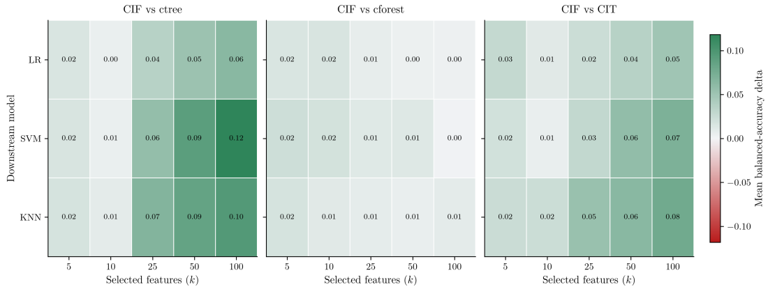
Figure 3: Classification CIF margins against ctree, cforest, and CIT by downstream learner and value of k . Each plotted value is the mean balanced-accuracy difference, CIF minus comparator, for one downstream learner and one value of k ; positive values favor CIF. Dataset counts by k are 21, 20, 14, 14, and 13 for ctree, 22, 21, 15, 15, and 14 for cforest, and 23, 22, 16, 16, and 15 for CIT. Values are means over datasets; the bootstrap intervals for the pooled differences are in Table 3.
