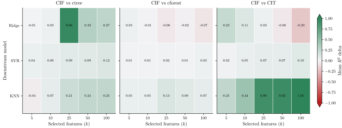
Figure 7: Regression CIF margins against ctree, cforest, and CIT by downstream learner and value of k . Each plotted value is the mean R^2 difference, CIF minus comparator, for one downstream learner and one value of k ; positive values favor CIF. Dataset counts by k are 8, 8, 7, 7, and 6 for each comparison. Large positive plotted values can reflect negative mean R^2 for the comparator. Numeric labels show the unclipped values; the color scale is clipped at \pm 1 for readability. Values are means over datasets; the bootstrap intervals for the pooled differences are in Table 20.
