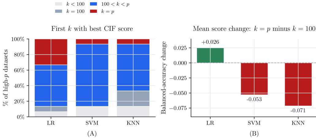
Figure 4: Where CIF’s classification scores peak as k increases, by downstream learner. (A) shows, for each learner, the percentage of 15 datasets where the first evaluated k attaining the best observed CIF score falls below 100, at 100, between 100 and p , or at k = p . (B) shows the mean balanced accuracy change from k = 100 to k = p .
