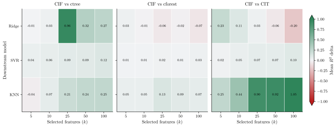
Figure 3: Regression CIF margins against ctrees, cforest, and CIT by downstream learner and value of k . Each plotted value is the mean R^2 difference, CIF minus comparator, for one downstream learner and one value of k ; positive values favor CIF. Dataset counts by k are 8, 8, 7, 7, and 6 for each comparison. Large positive plotted values can reflect negative mean R^2 for the comparator. Numeric labels show the unclipped values; the color scale is clipped at \pm 1 for readability. Values are means over datasets; the bootstrap intervals for the pooled differences are in Table 3.
