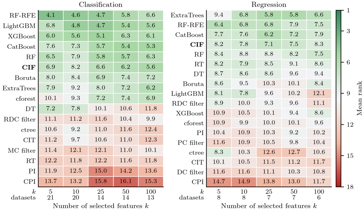
Figure 1: Mean rank of every feature selection method by the number of selected features k , for classification (left, 17 methods) and regression (right, 18 methods), averaged across downstream models at each value of k ; lower ranks are better, and the two panels share one colour scale. Each column uses the datasets on which every method has results at that k , whose number is given under k .
