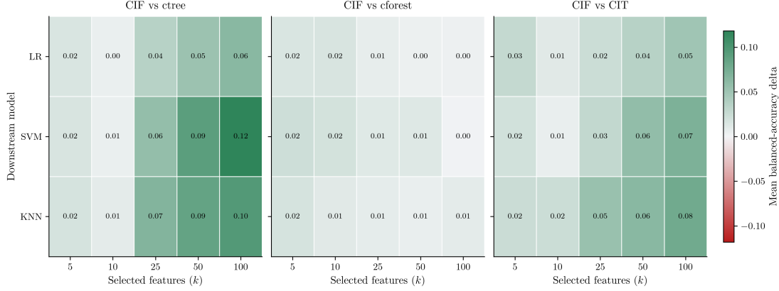
Figure 2: Classification CIF margins against ctrees, cforest, and CIT by downstream learner and value of k . Each plotted value is the mean balanced-accuracy difference, CIF minus comparator, for one downstream learner and one value of k ; positive values favor CIF. Dataset counts by k are 21, 20, 14, 14, and 13 for ctrees, 22, 21, 15, 15, and 14 for cforest, and 23, 22, 16, 16, and 15 for CIT. Values are means over datasets; the bootstrap intervals for the pooled differences are in Table 3.
