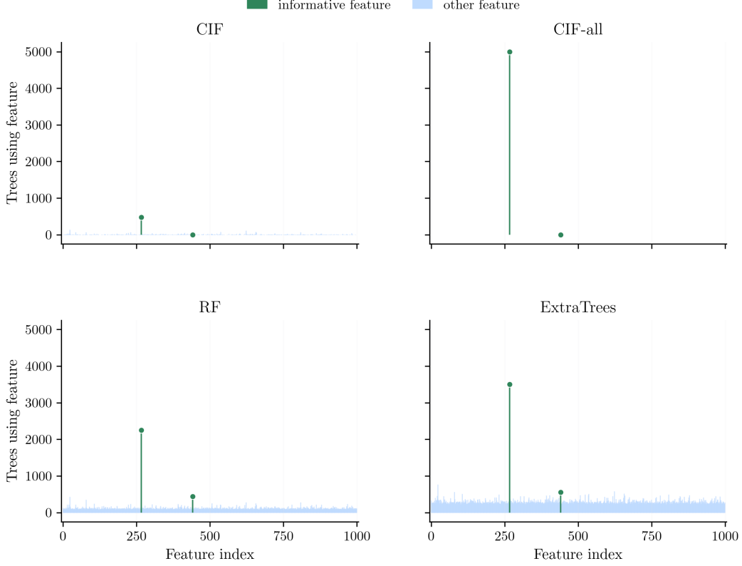
Figure 6: Tree-level feature use in one sparse classification forest design ( n = 250 , p = 1,000 , two informative features). Counts are the number of trees using each feature in at least one split, pooled over five fits of 1,000 trees each, so the shared vertical axis runs to 5,000. CIF samples a subset of features at each node; CIF-all evaluates all nonconstant features.
