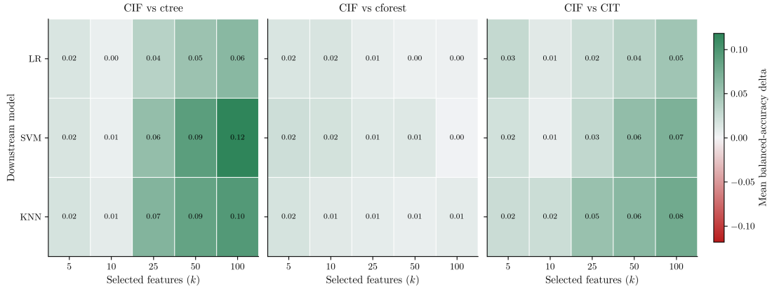
Figure 3: Classification CIF margins against ctree, cforest, and CIT by downstream learner and value of k . Each plotted value is the mean balanced-accuracy difference, CIF minus comparator, for one downstream learner and one value of k ; positive values favor CIF. Dataset counts by k are 21, 20, 14, 14, and 13 for ctree, 22, 21, 15, 15, and 14 for cforest, and 23, 22, 16, 16, and 15 for CIT. Values are means over datasets; the bootstrap intervals for the pooled differences are in Table 3.
