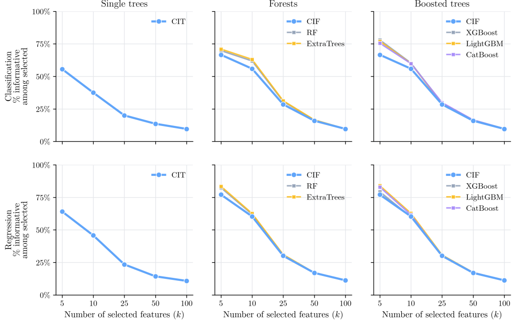
Figure 6: Synthetic top- k recovery curves. Columns compare single trees, forests, and boosted trees; rows show classification and regression. Each value is the percentage of selected features that are truly informative.
