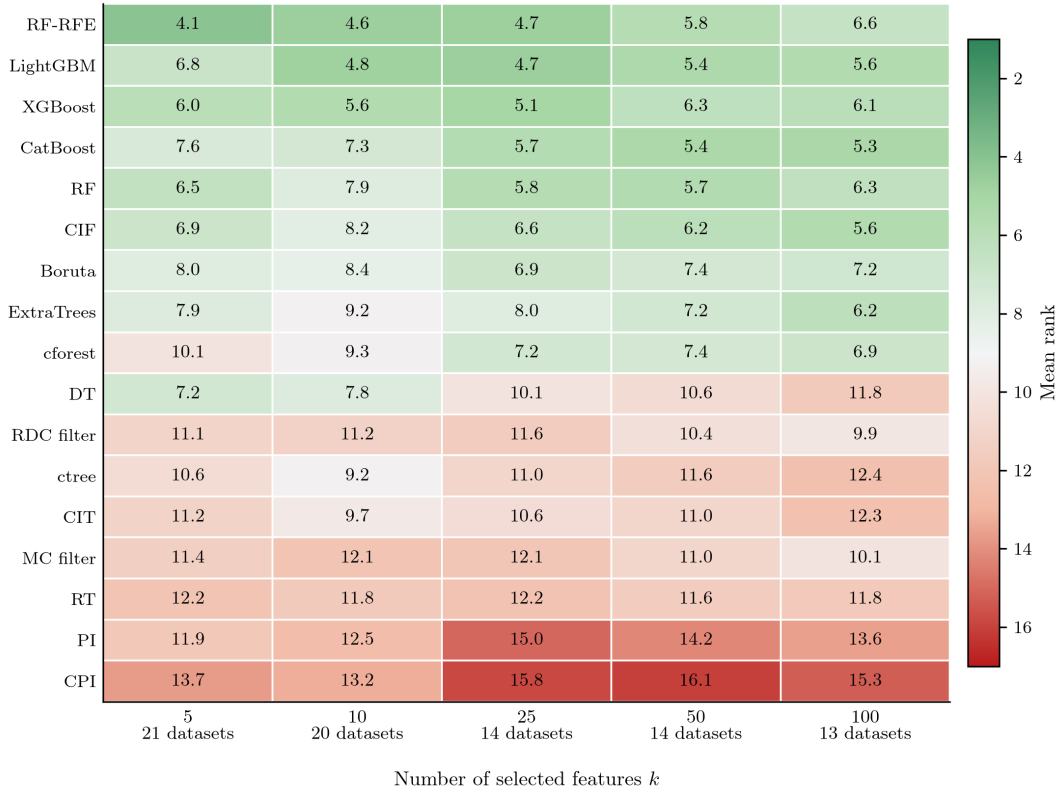
Figure 1: Classification mean rank by number of selected features. Rows show all 17 feature selection methods, averaged across downstream models at each value of k ; lower ranks are better. The columns for k = 5, 10, 25, 50, 100 use 21, 20, 14, 14, and 13 datasets.
