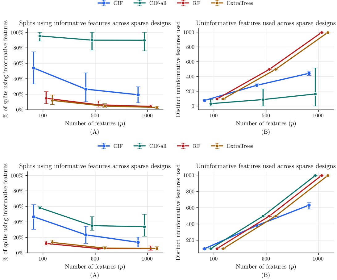
Figure 8: Forest feature use by feature dimension p , for classification (top row) and regression (bottom row), with 1,000 trees per fit. Points are means over n_{\text{informative}} \in \{1, 2, 5, 10\} ; capped bars span the minimum and maximum over those four sparse designs. In each row, (A) shows the percentage of splits using informative features and (B) the number of distinct uninformative features used. CIF samples a subset of features at each node; CIF-all evaluates all nonconstant features.
