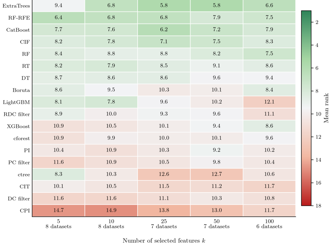
Figure 2: Regression mean rank by number of selected features. Rows show all 18 feature selection methods, averaged across downstream models at each value of k ; lower ranks are better. The columns for k = 5, 10, 25, 50, 100 use 8, 8, 7, 7, and 6 datasets.
