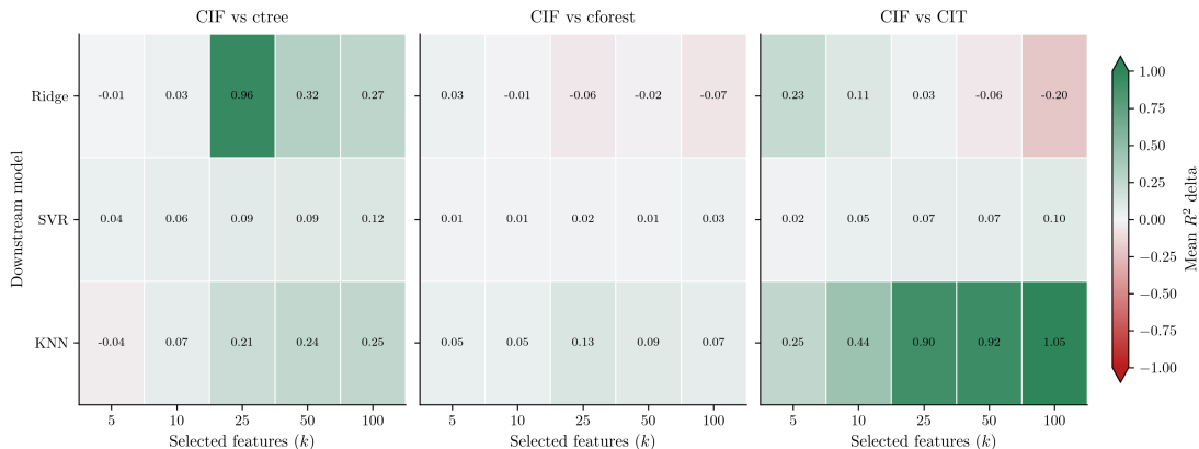
Figure 4: Regression CIF margins against ctrees, cforest, and CIT by downstream learner and value of k . Each plotted value is the mean R^2 difference, CIF minus comparator, for one downstream learner and one value of k ; positive values favor CIF. Dataset counts by k are 8, 8, 7, 7, and 6 for each comparison. Large positive plotted values can reflect negative mean R^2 for the comparator. Numeric labels show the unclipped values; the color scale is clipped at \pm 1 for readability. Values are means over datasets; the bootstrap intervals for the pooled differences are in Table 3.
