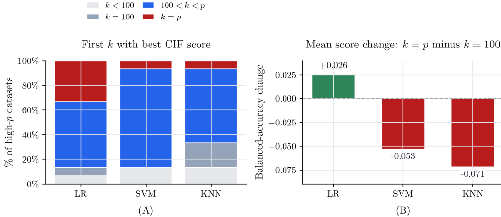
Figure 5: Where CIF’s classification scores peak as k increases, by downstream learner. (A) shows, for each learner, the percentage of 15 datasets where the first evaluated k attaining the best observed CIF score falls below 100, at 100, between 100 and p , or at k = p . (B) shows the mean balanced accuracy change from k = 100 to k = p .
