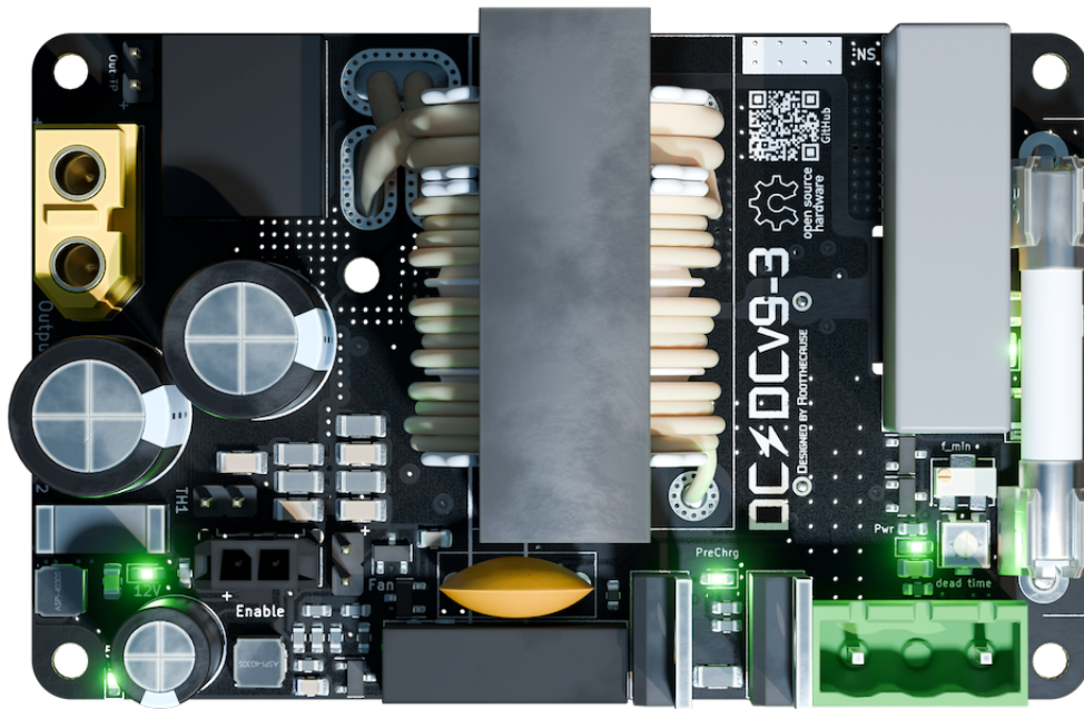
Figure 2: DCDC PCB design populated with components.
