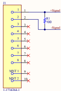
Differential Pair Input (RJ45 - CAT 5 | Non-shielded)
