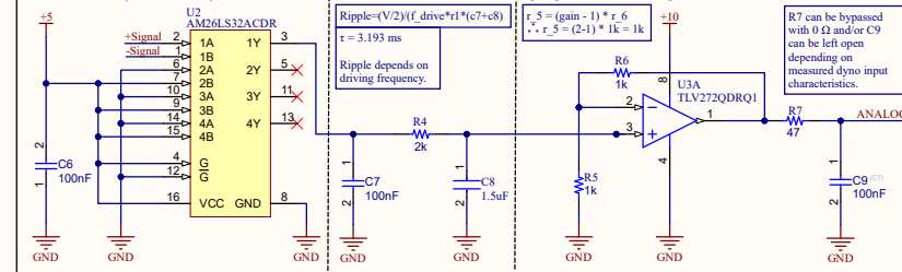
Differential Receiver (RS-422 Standard)
