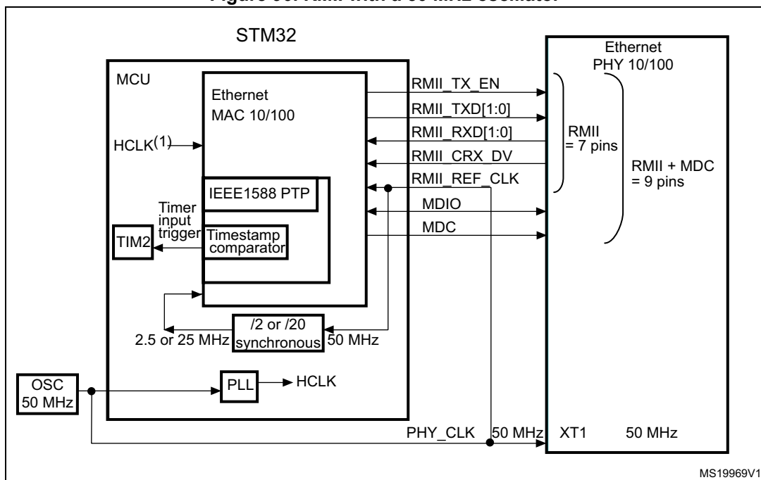
Figure 90. RMI with a 50 MHz oscillator
