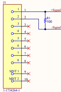
Differential Pair Input (RJ45 - CAT 5 | Non-shielded)
