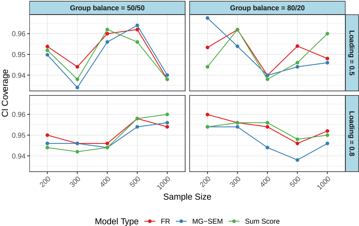
Confidence Interval Coverage | RSQ_prod = 0, items = 6
