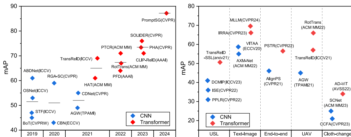
Fig. 1 (1) We show the performance of recent state-of-the-art methods on the widely-used person Re-ID dataset MSMT17 (left). The transformer-based methods have achieved a comprehensive lead in accuracy since 2021, while the CNN-based method for single-modal image Re-ID has not been studied. (2) We show state-of-the-art results
