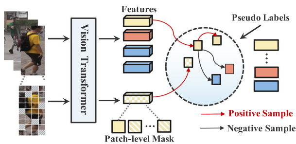
Fig. 7 The proposed unsupervised Transformer baseline for Re-ID enhanced with a patch-level mask learning strategy
