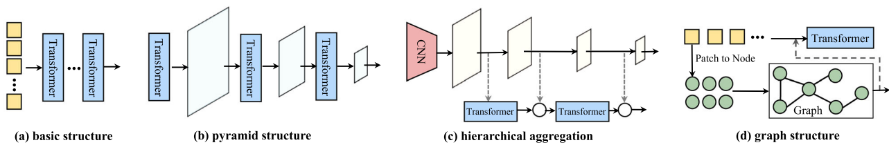
Fig. 5 Different transformer architectures designed for image-based Re-ID. a The basic Re-ID baseline based on Vision Transformer (He et al., 2021a). b Pyramid Transformer for learning multi-scale features (Li
