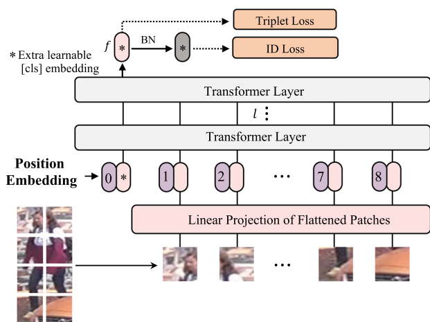
Fig. 4 The first pure transformer baseline for object Re-ID (He et al., 2021a). The Vision Transformer backbone (Dosovitskiy et al., 2020) is adopted as a feature extractor, optimized with ID loss and triplet loss (Hermans et al., 2017) widely used in Re-ID
