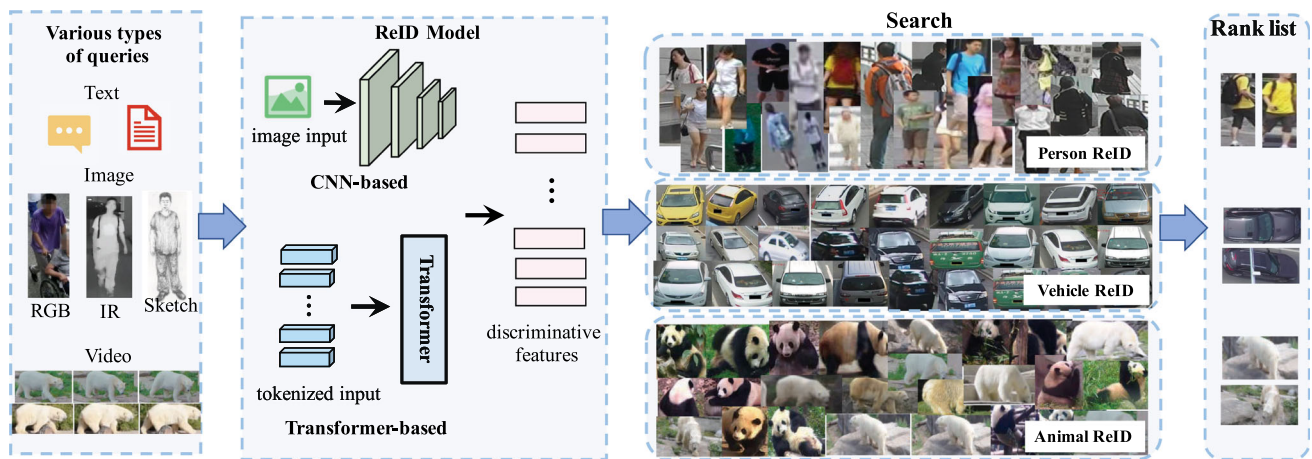
Fig. 3 General object Re-ID process. Given a query that can be any type of image, text, video, etc. , the goal of Re-ID is to search for the specific object from gallery data collected by different cameras
