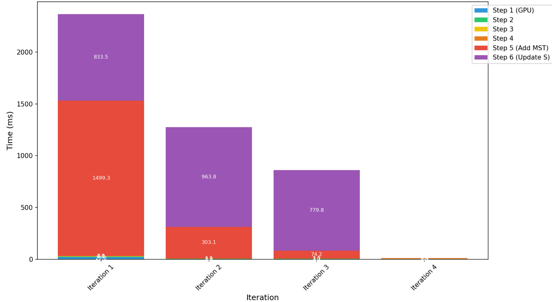
MST Algorithm - Time Distribution by Iteration
