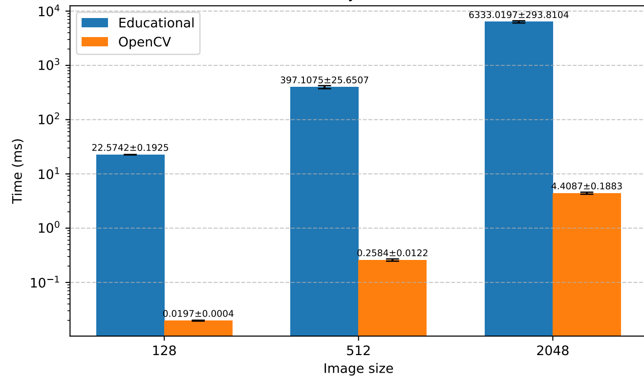
gaussian_blur_5x5 zero_padding (Rgb)
