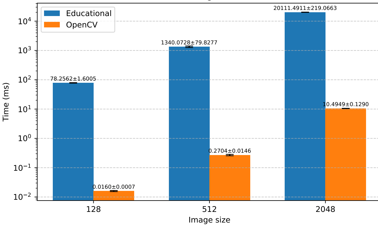
sharpen_3x3 replicate_padding (Rgb)
