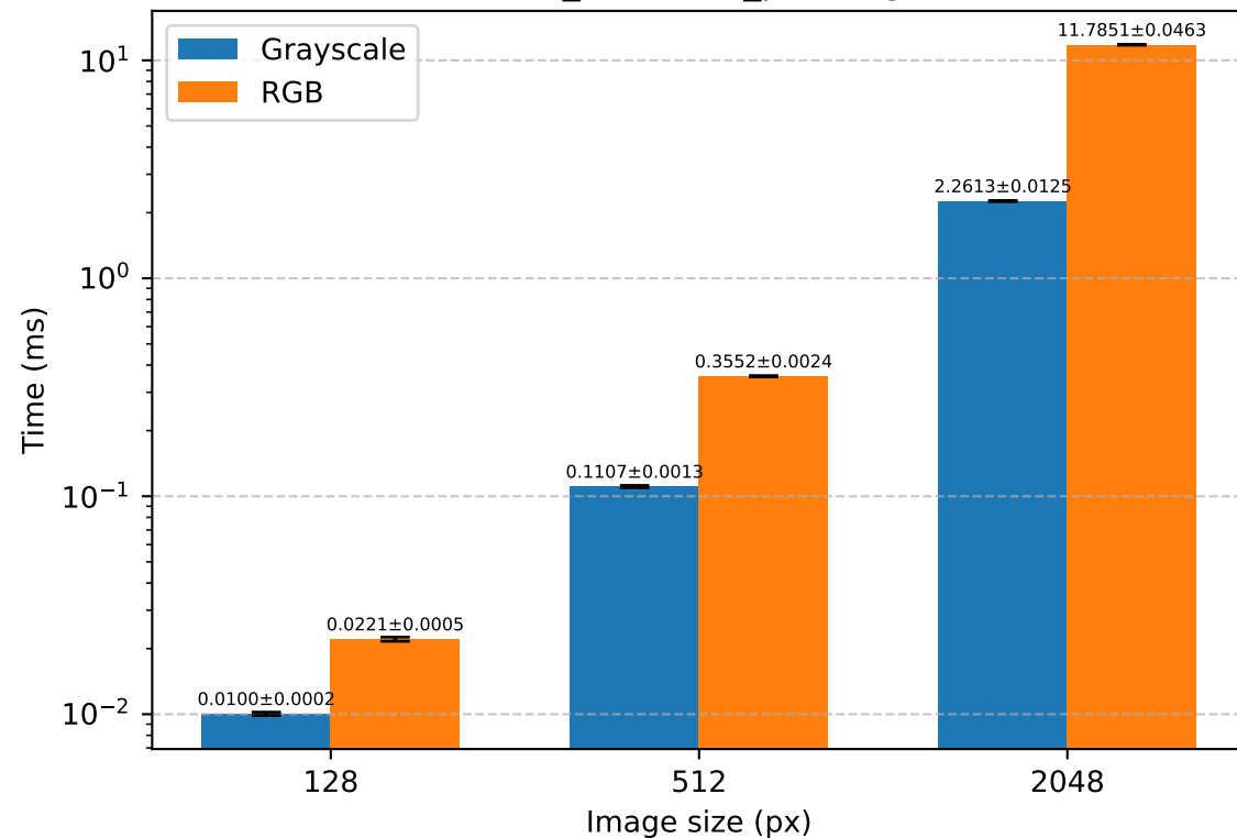
OpenCV (cv2.filter2D) blur_3x3, zero_padding
