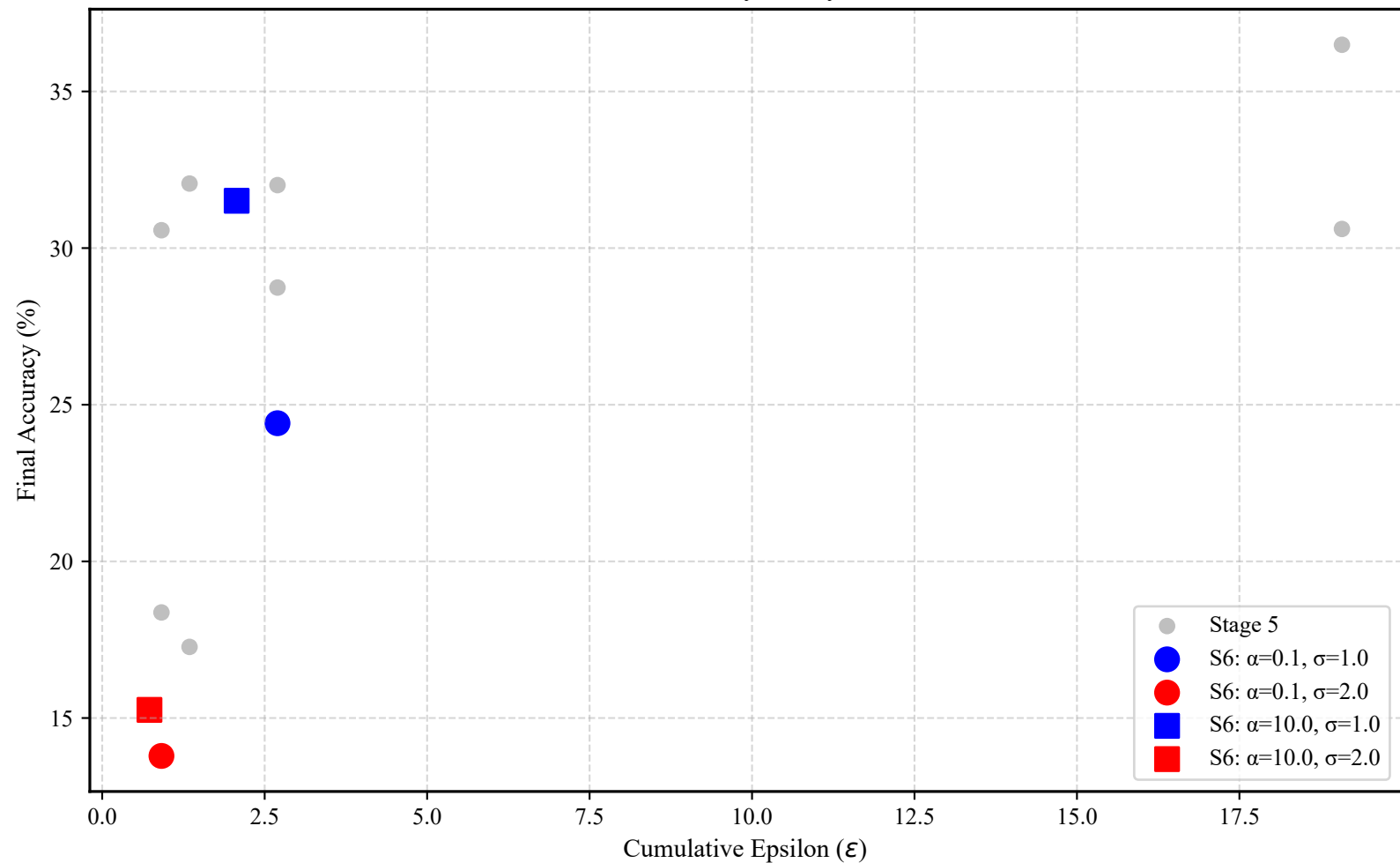
Combined Privacy-Utility Tradeoff
