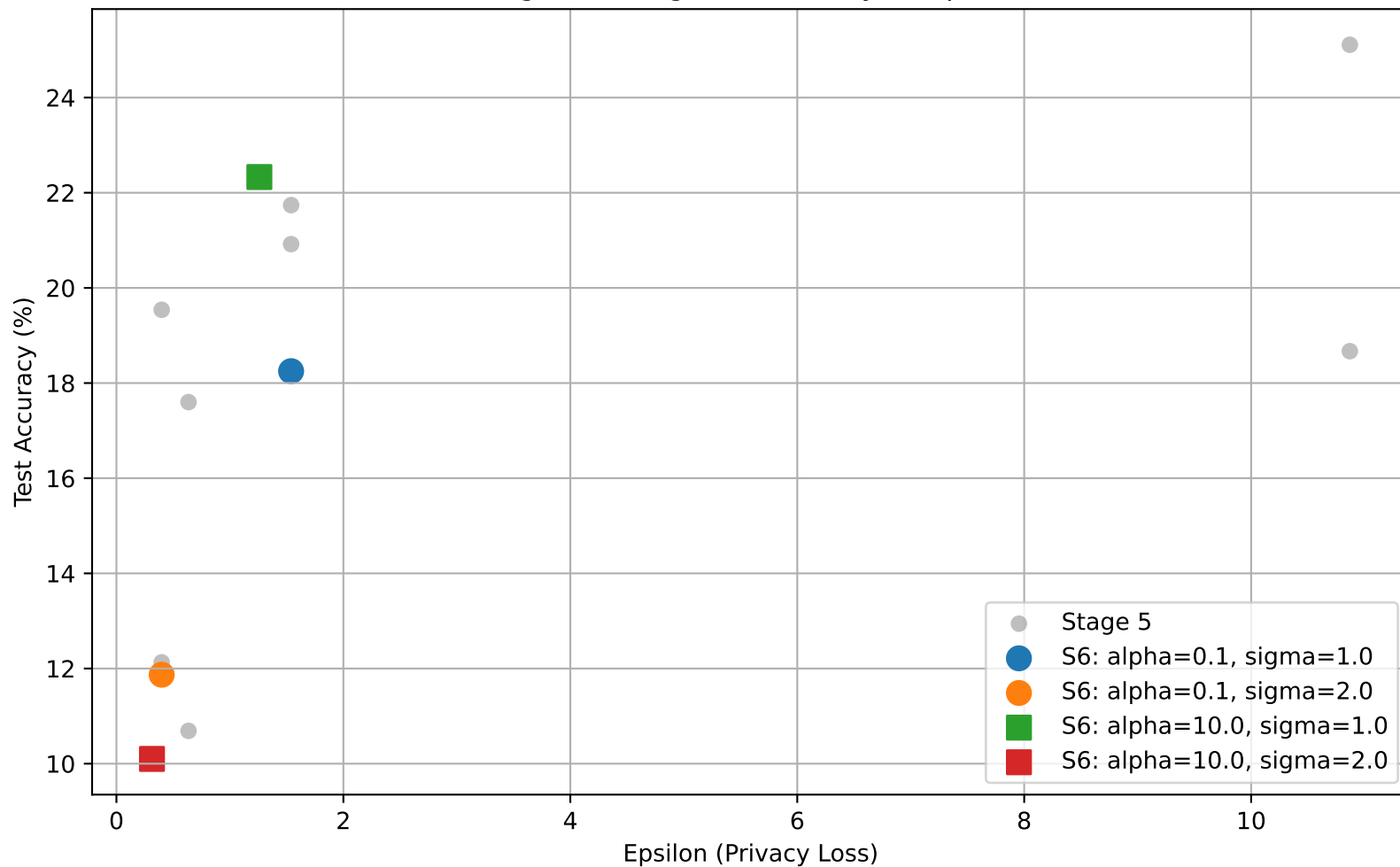
Stage 5 & Stage 6: Accuracy vs Epsilon
