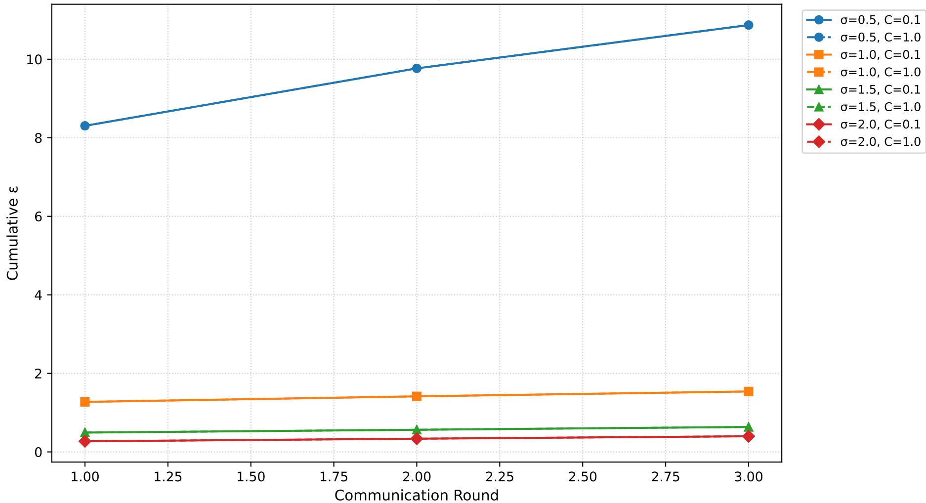
Cumulative \epsilon per Communication Round Full CIFAR-10 | \delta=1e-5
