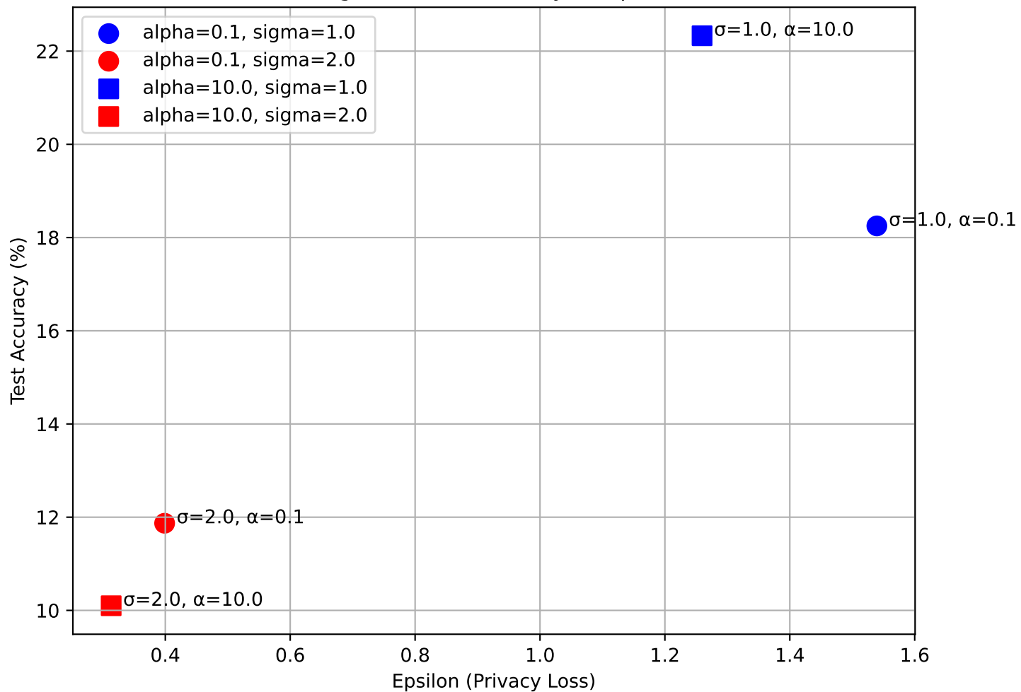
Stage 6: Final Accuracy vs Epsilon
