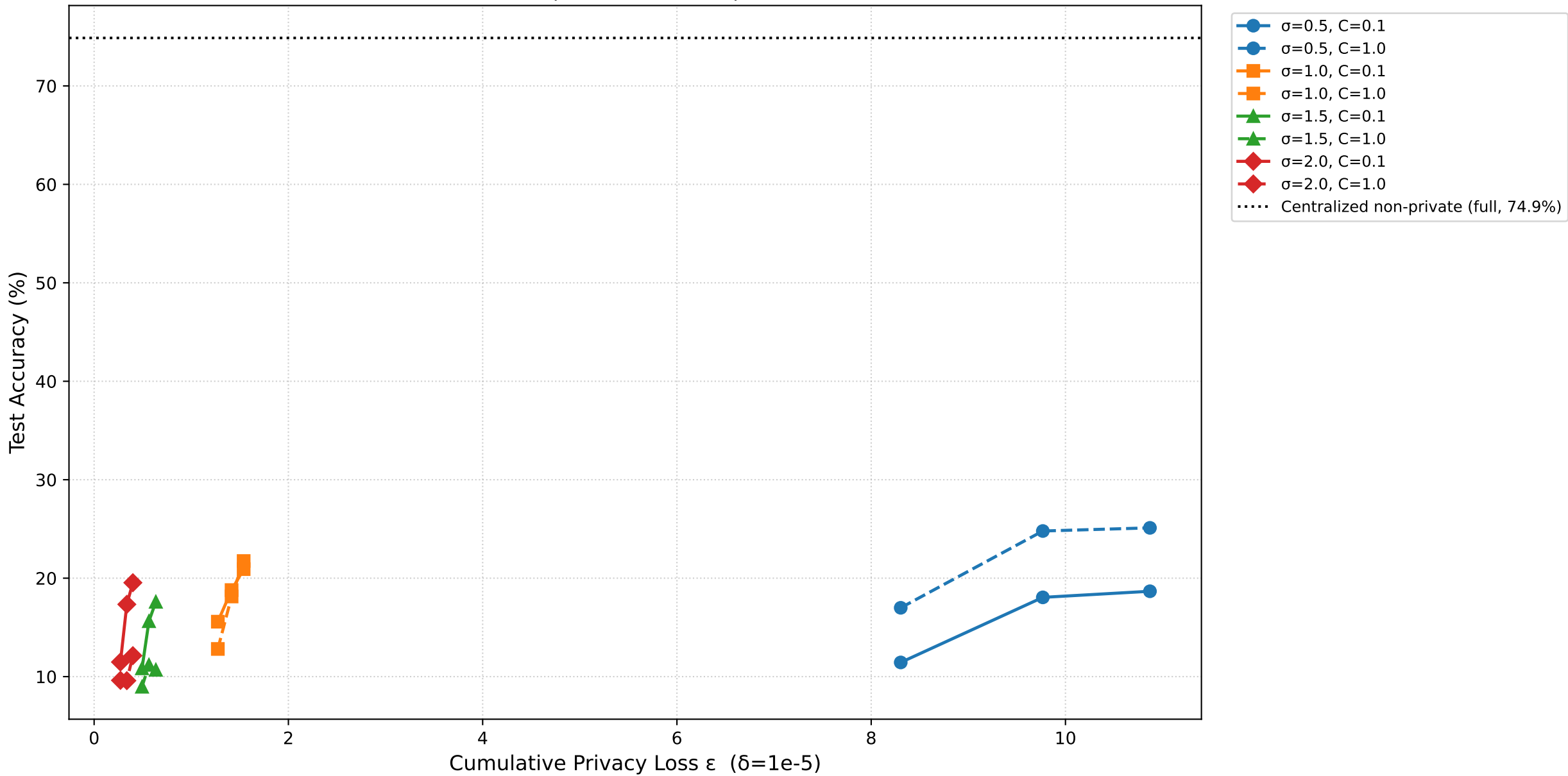
Privacy-Utility Tradeoff Accuracy vs Cumulative \epsilon | Full CIFAR-10 | \delta=1e-5 , Dirichlet \alpha=0.1
