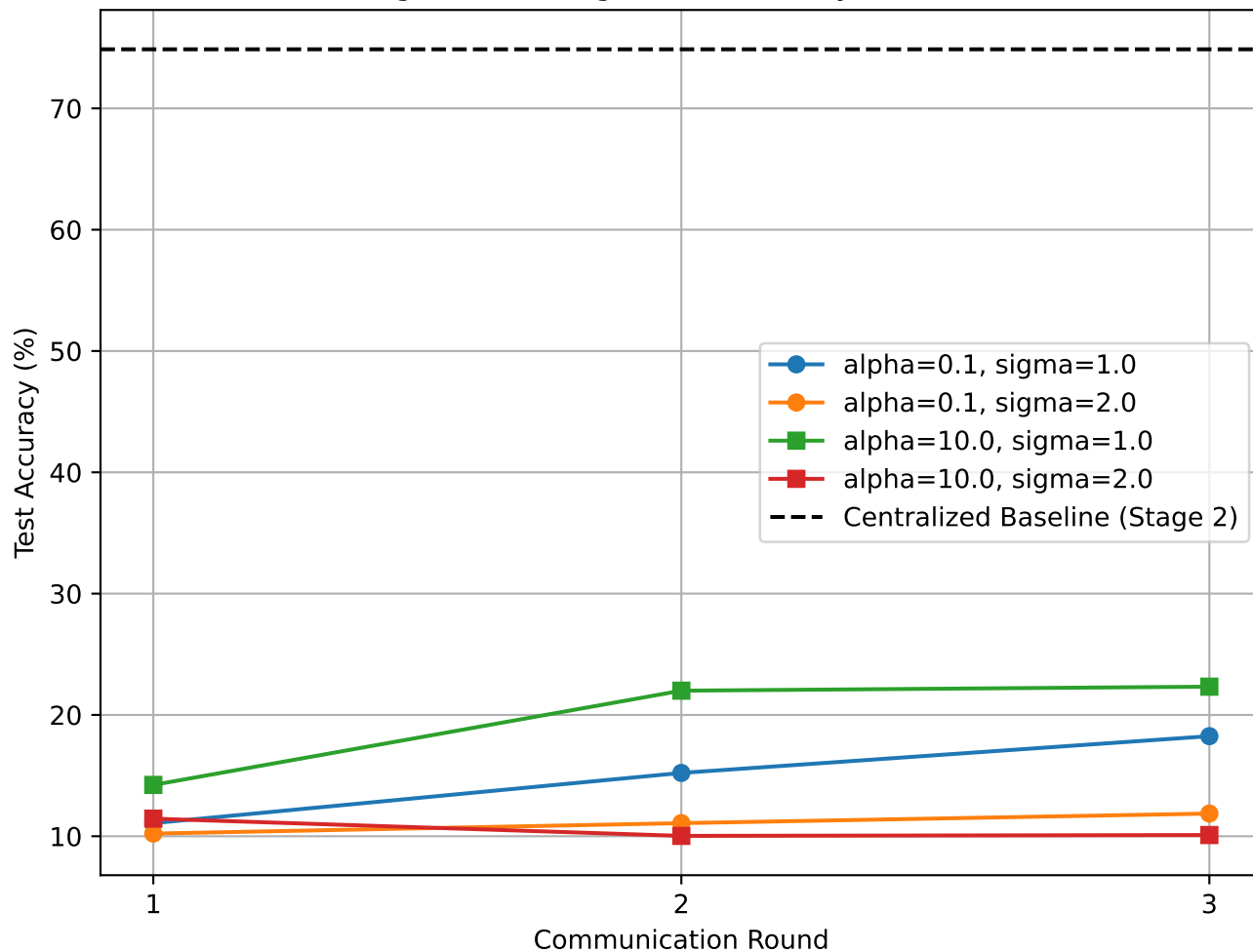
Stage 6: Convergence (Accuracy vs Round)
