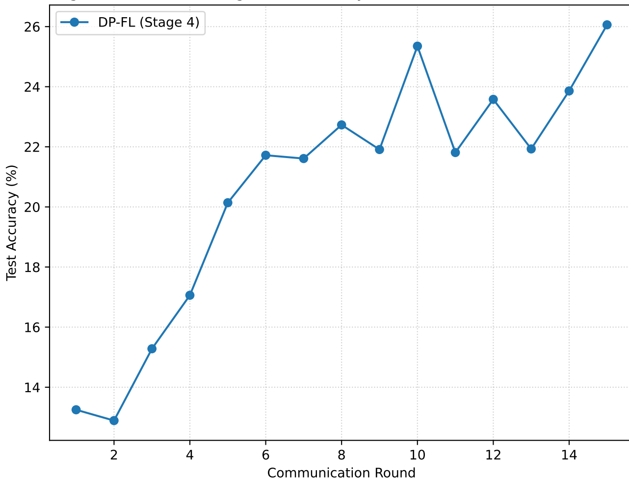
Figure 2: DP-FL Convergence (Accuracy vs Round) (SUBSET VALIDATION)
