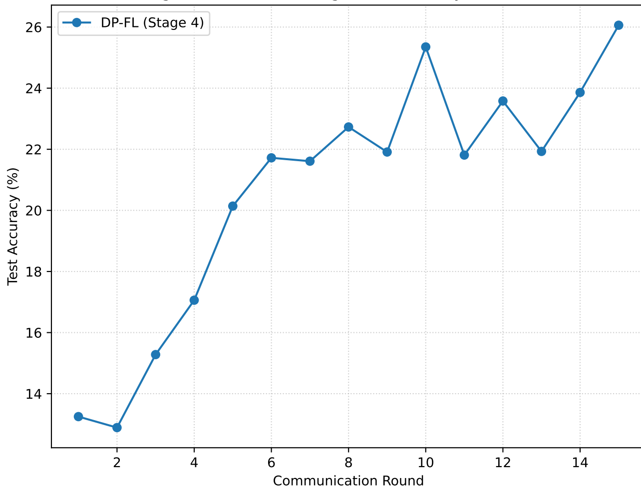
Figure 2: DP-FL Convergence (Accuracy vs Round)
