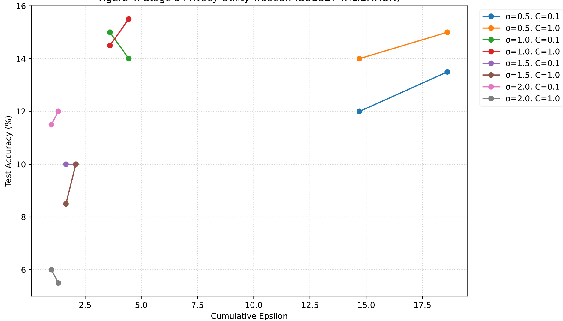
Figure 4: Stage 5 Privacy-Utility Tradeoff (SUBSET VALIDATION)
