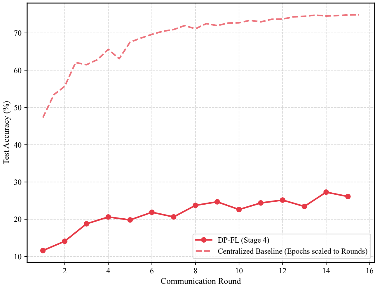
Stage 4 DP-FL Accuracy Convergence
