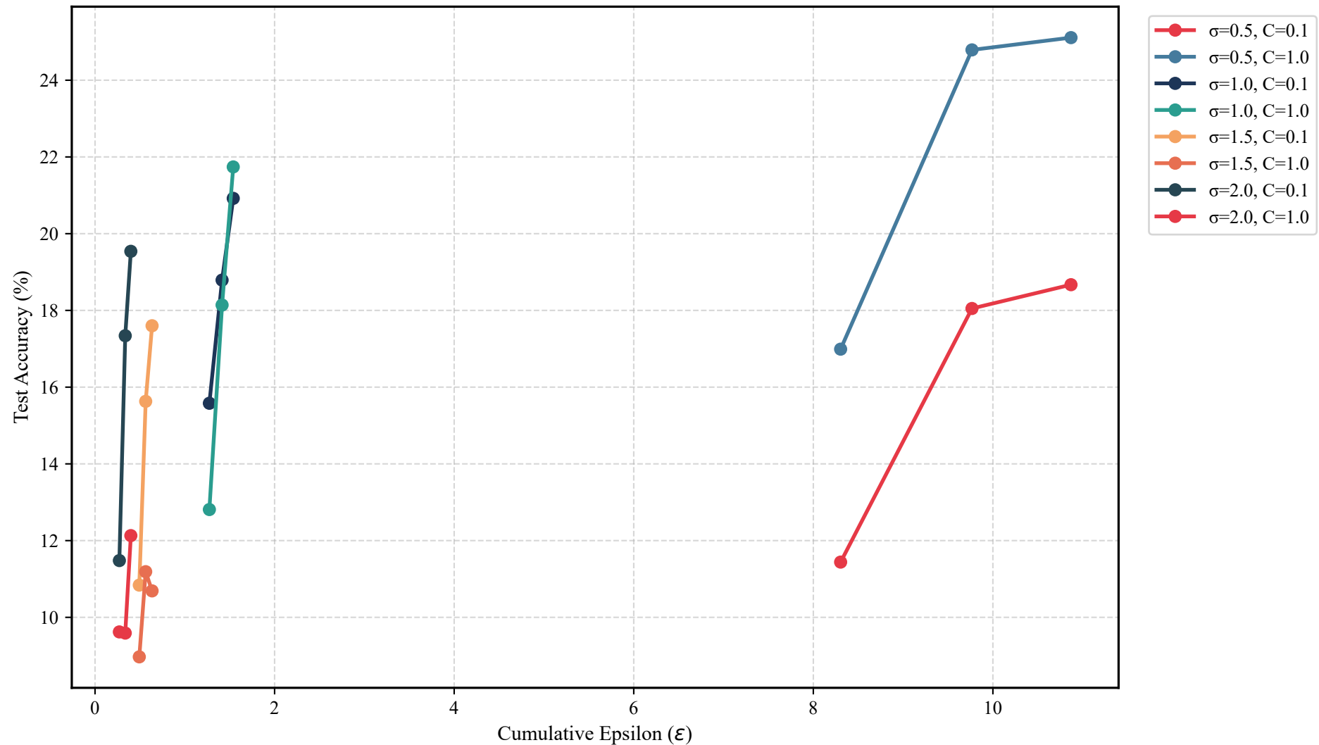
Stage 5 Privacy-Utility Tradeoff
