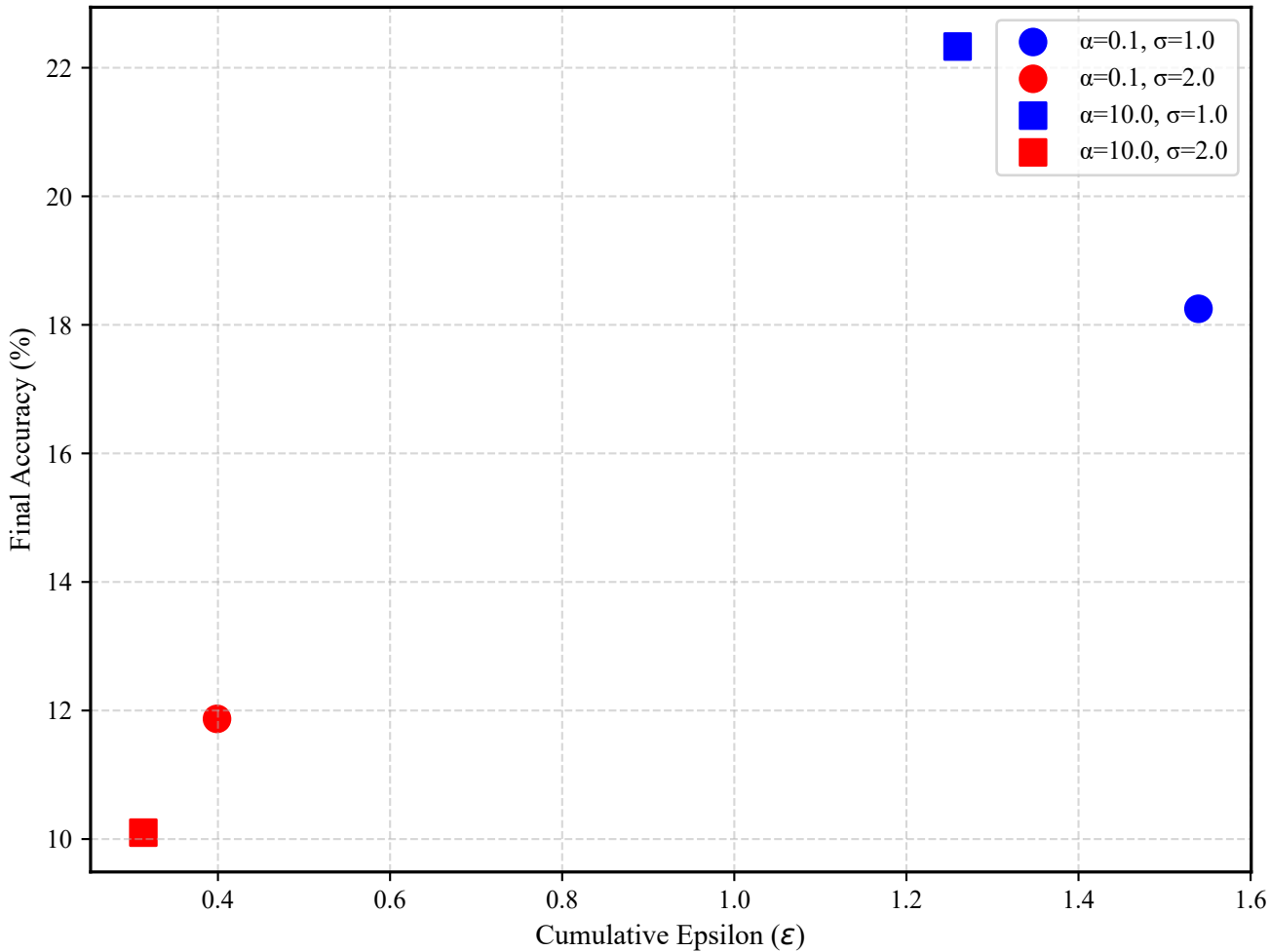
Stage 6 Alpha/Sigma Ablation
