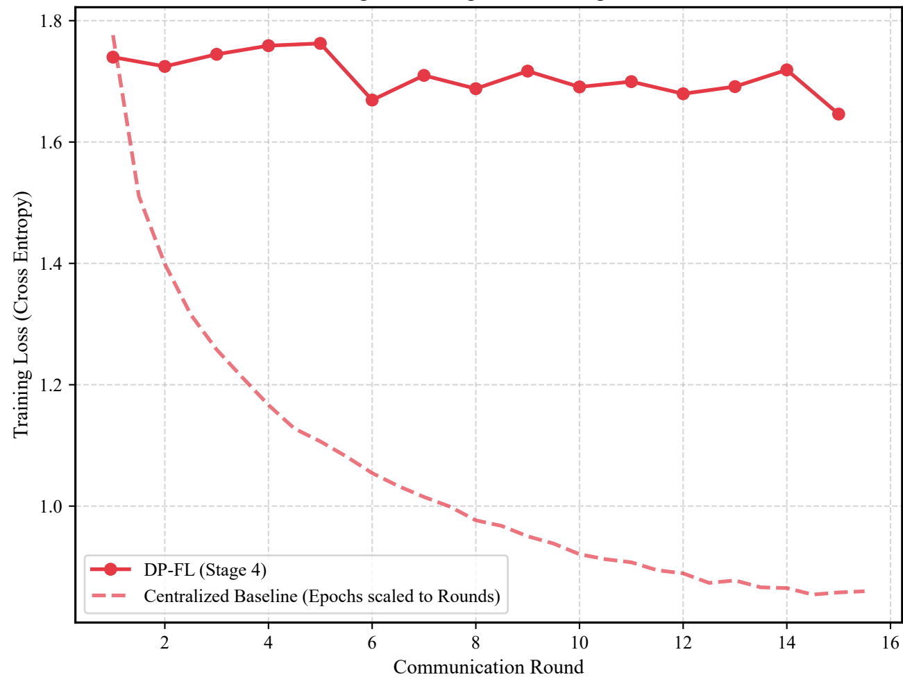
Stage 4 Training Loss Convergence
