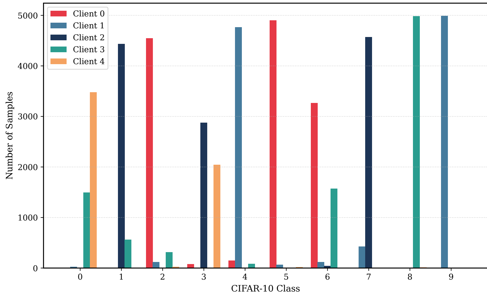
Client Label Distribution under Dirichlet \alpha=0.1
