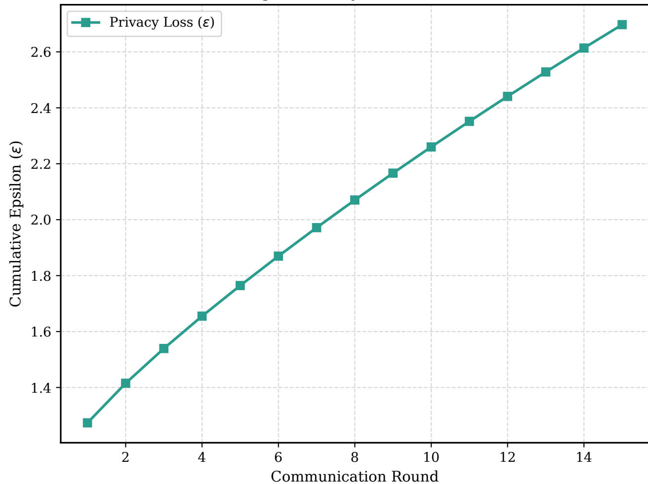
Stage 4 Privacy Accumulation
