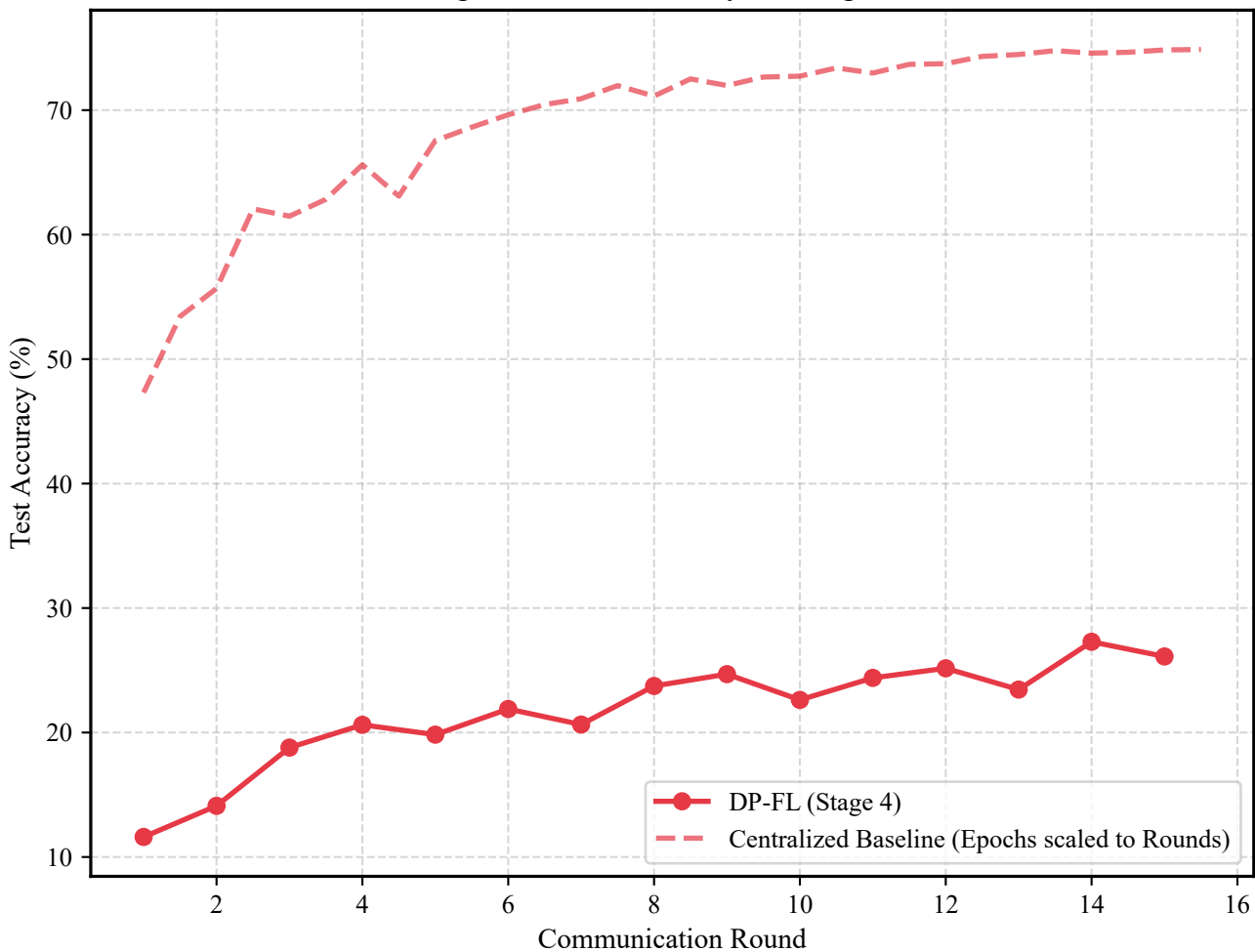
Figure 2a: Test Accuracy Convergence
