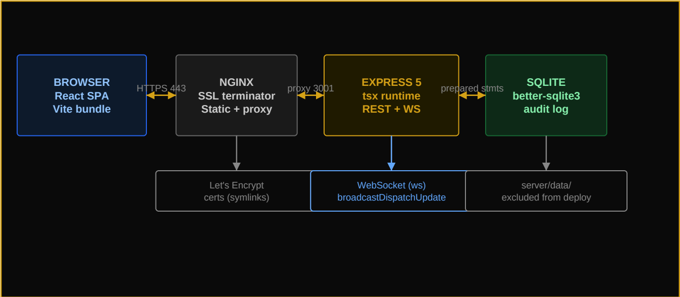
Fig. C-1 — RMPG Flex system architecture. Browser -> nginx -> Express -> SQLite.
