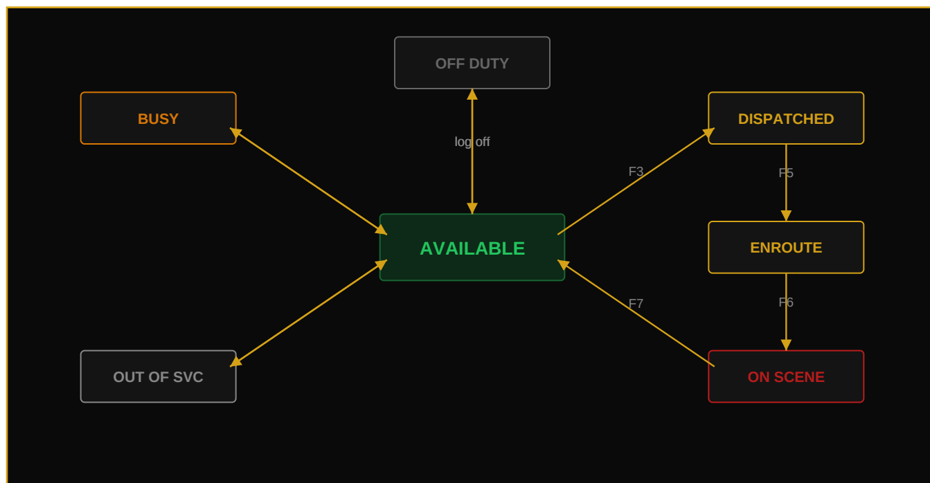
Fig. 3-1 — Legal unit status transitions. AVAILABLE is the hub; illegal transitions are blocked by the server.
