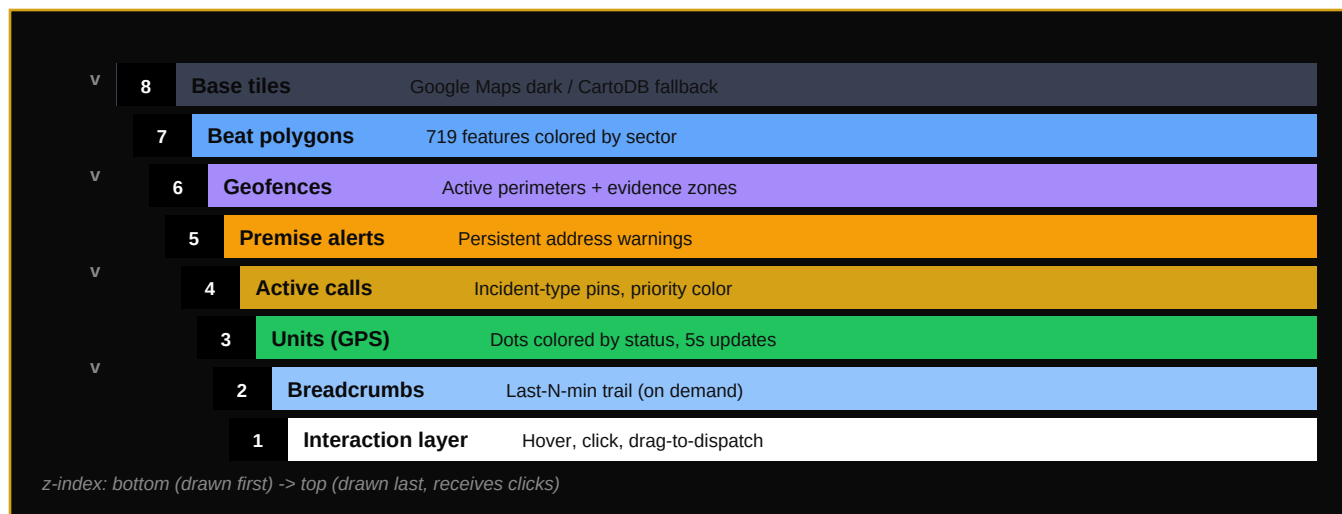
Fig. 12-1 — Map layer stack on /map. Interaction layer is always on top.
