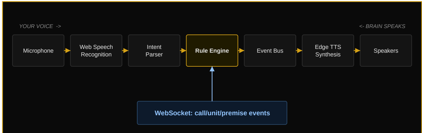
Fig. 7-1 — Dispatcher Brain signal flow. Rule Engine fires on both your speech AND live system events.
