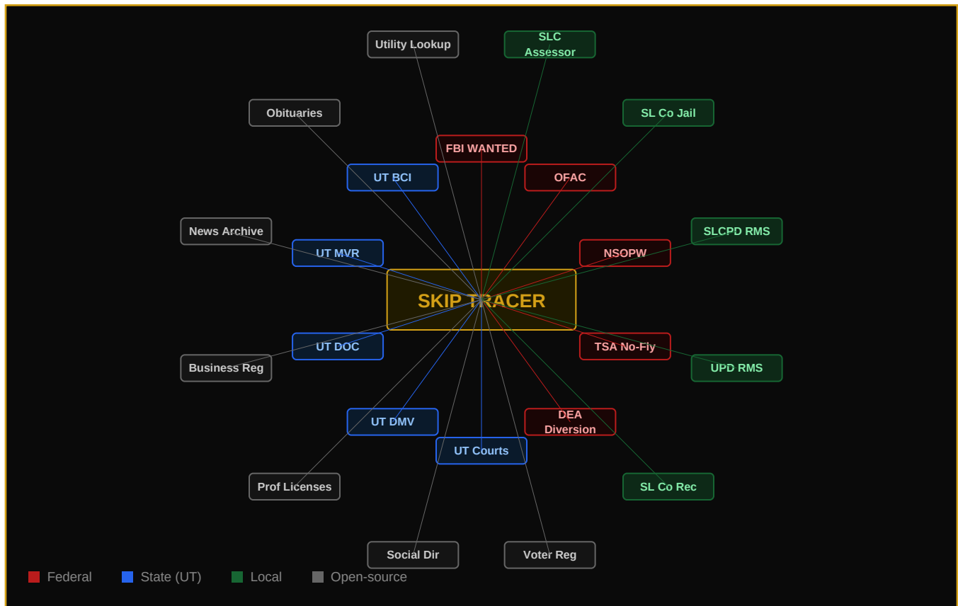
Fig. 18-1 — Skip Tracer V2 source fan-out. 22 parallel adapters grouped by jurisdiction.
