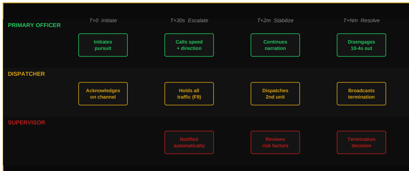
Fig. 8-1 — Pursuit swim-lane. Three roles work in parallel, not sequence.
