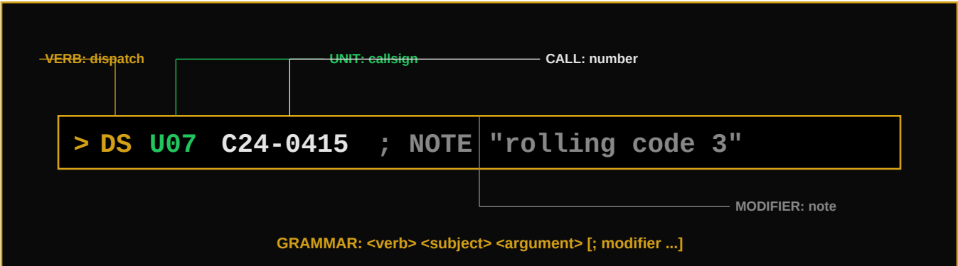
Fig. 6-1 — CAD command-line syntax. Tokens are space-separated; semicolons chain modifiers.
