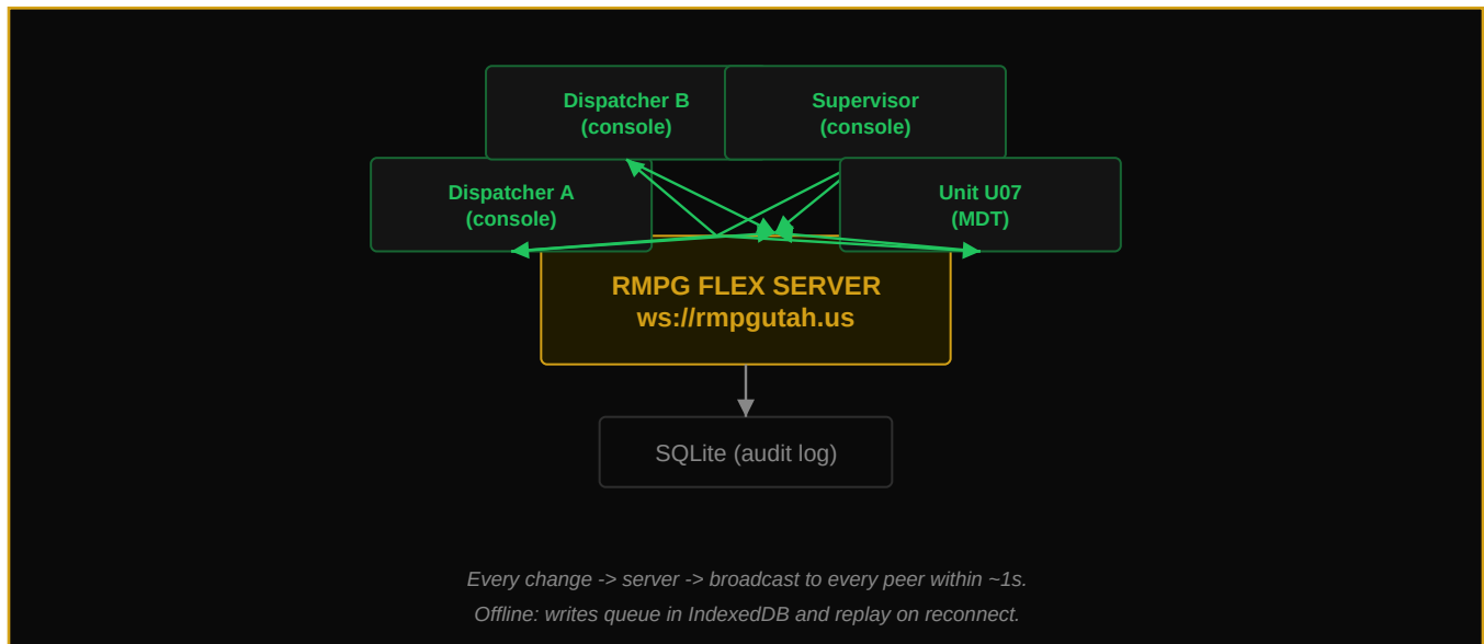
Fig. 14-1 — Real-time sync topology. Single server, N clients, WebSocket broadcast.
