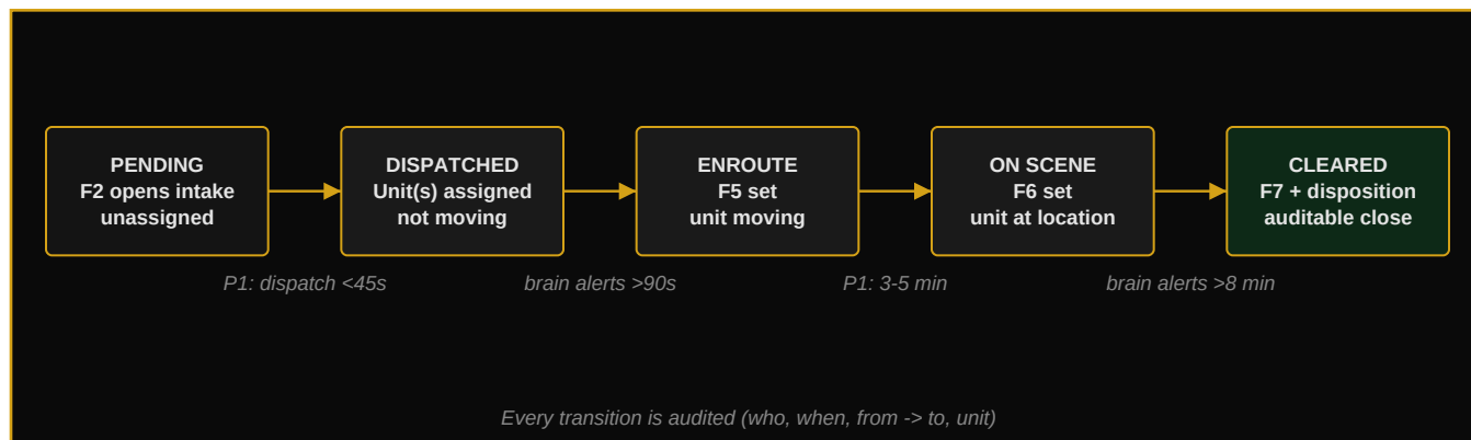
Fig. 2-1 — Call state lifecycle with typical transition timings.
