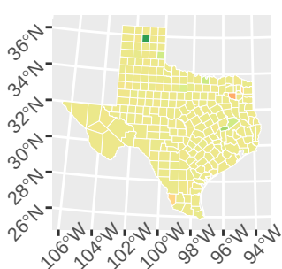
%Change in Random Effect
