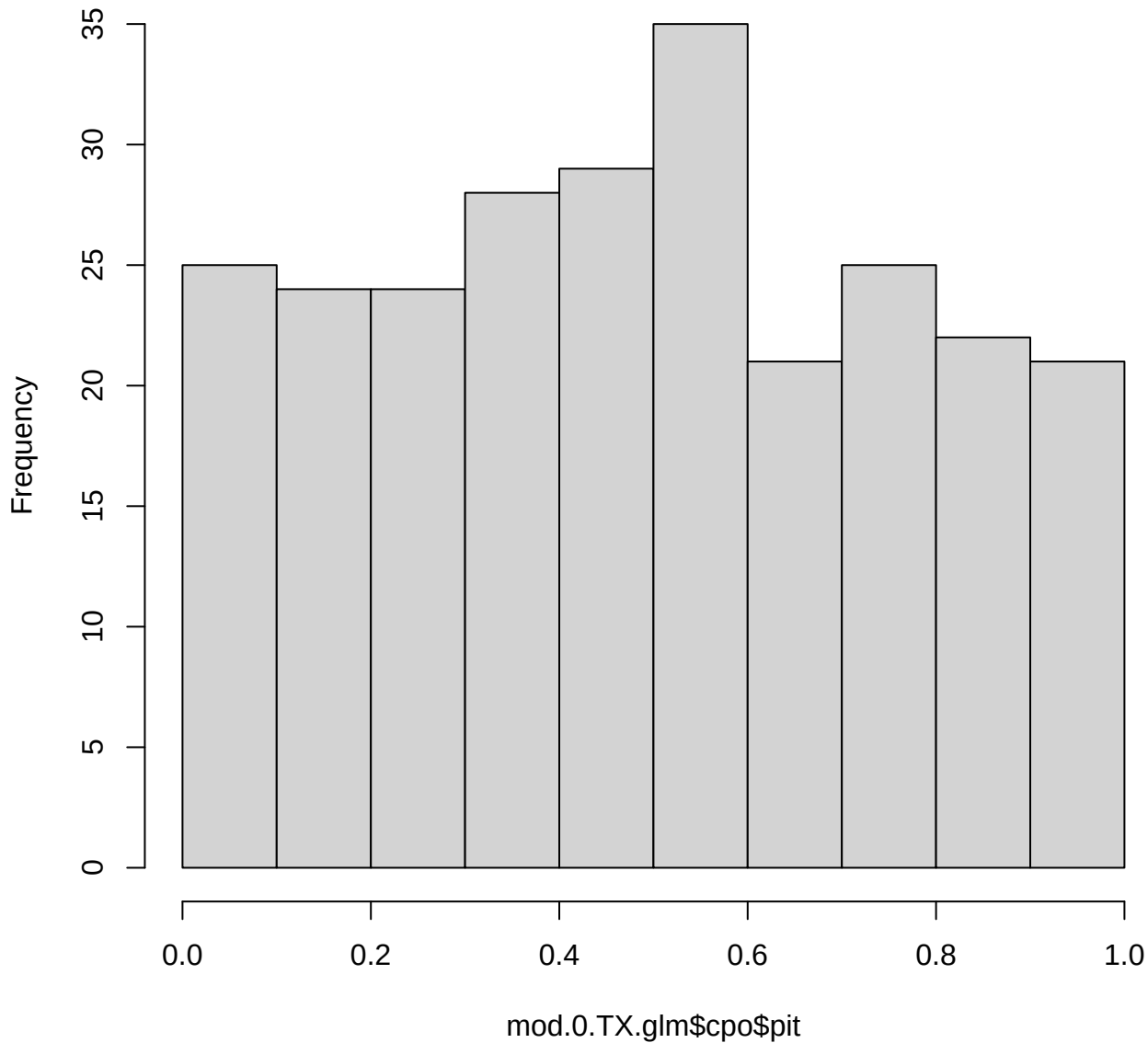
Histogram of mod.0.TX.glm$cpo$pit
