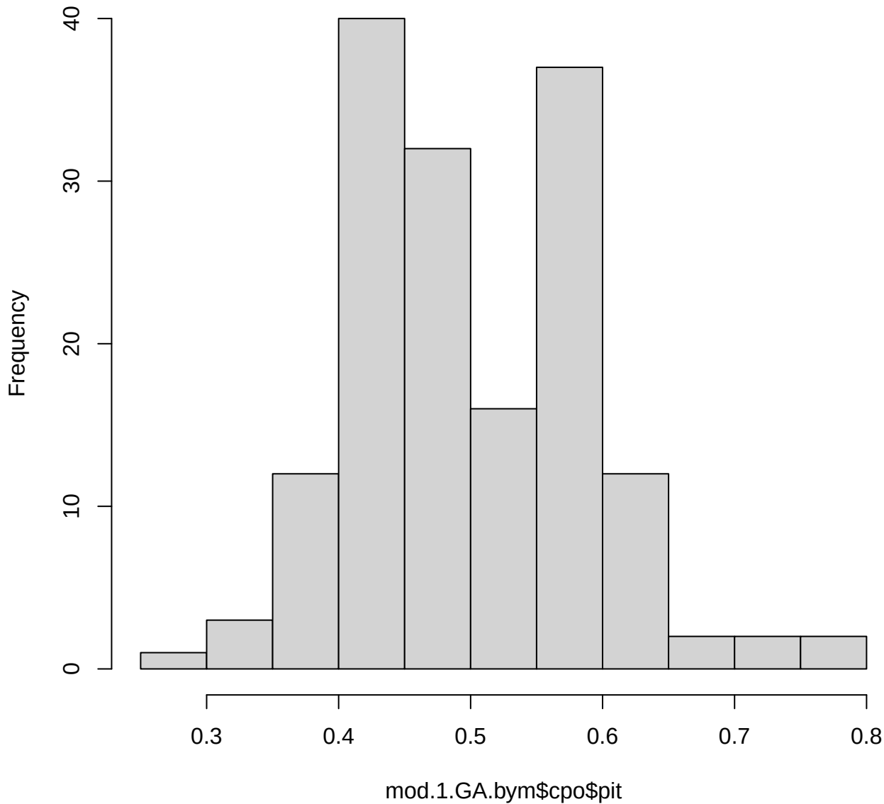
Histogram of mod.1.GA.bym$cpo$pit
