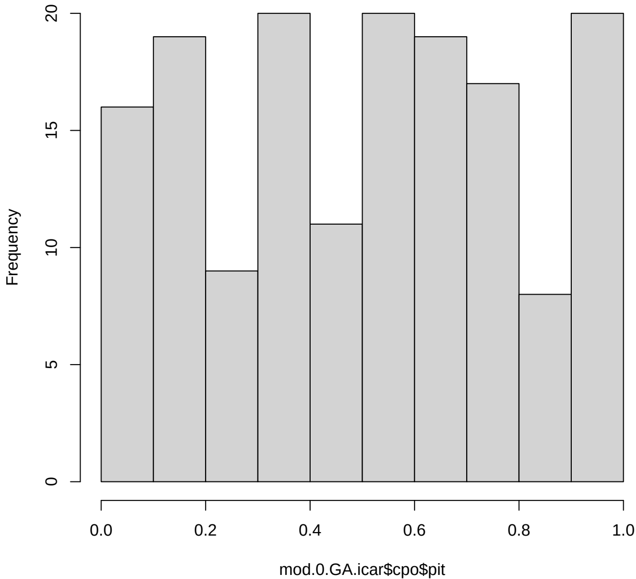
Histogram of mod.0.GA.icar$cpo$pit
