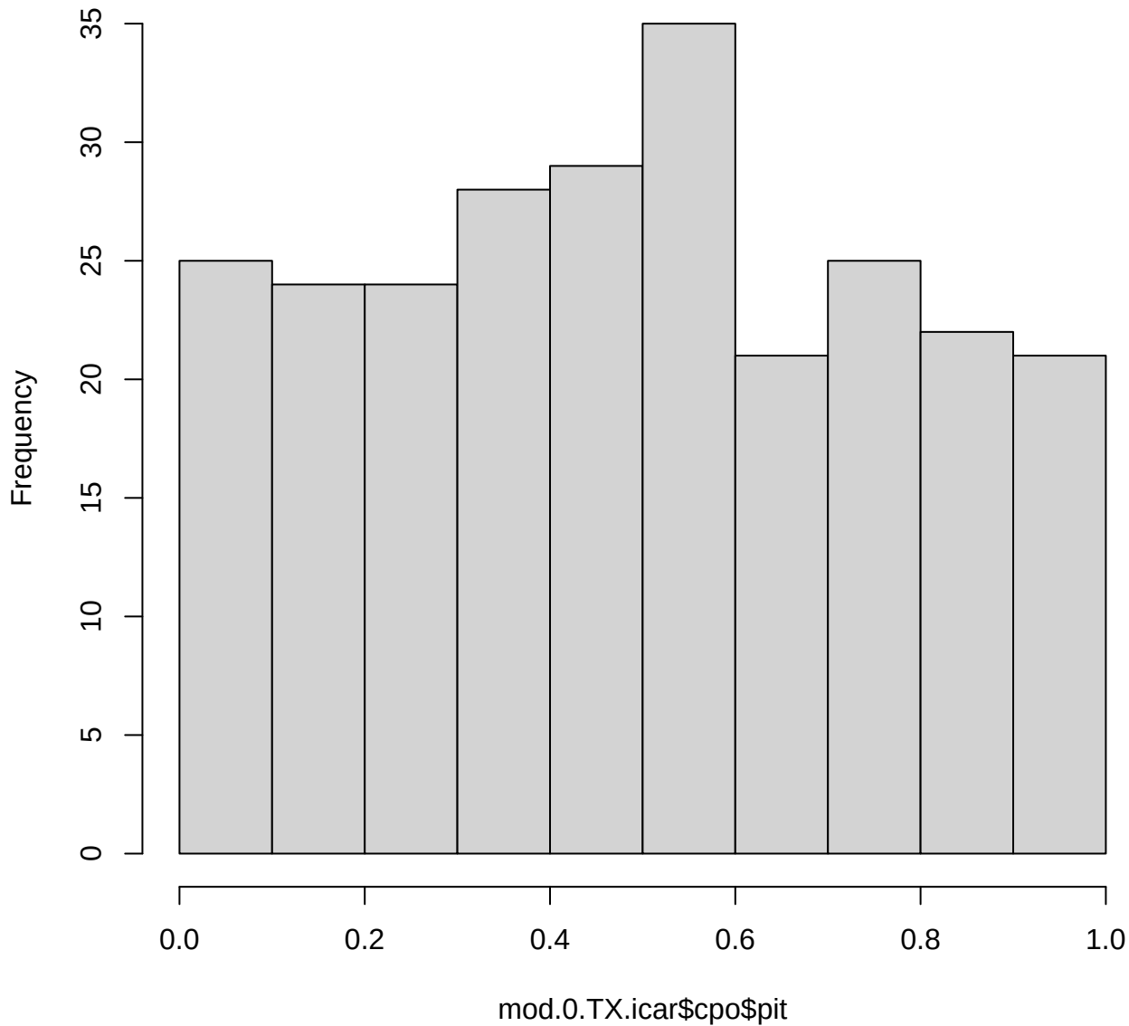
Histogram of mod.0.TX.icar$cpo$pit
