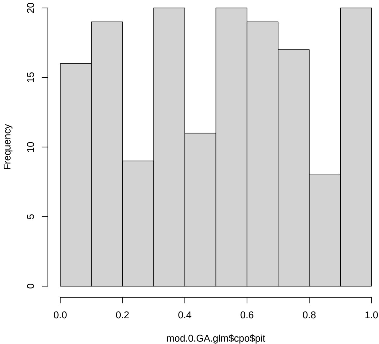
Histogram of mod.0.GA.glm$cpo$pit
