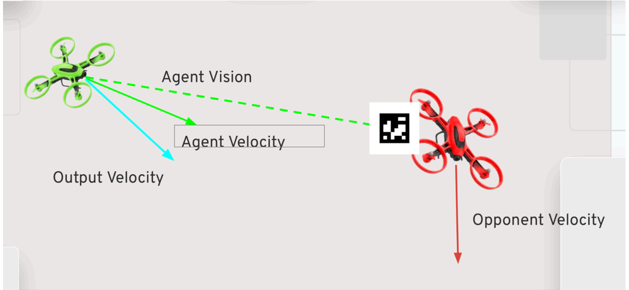
Figure 2. Observation geometry. The tracker (green) observes its own velocity, the opponent's velocity, and the opponent's relative position in its body frame. Its action is a 3D velocity command. The same nine-dimensional observation vector is fed at deployment, with AprilTag pose supplying the relative-position component and visual-flow differencing supplying the opponent velocity estimate.
