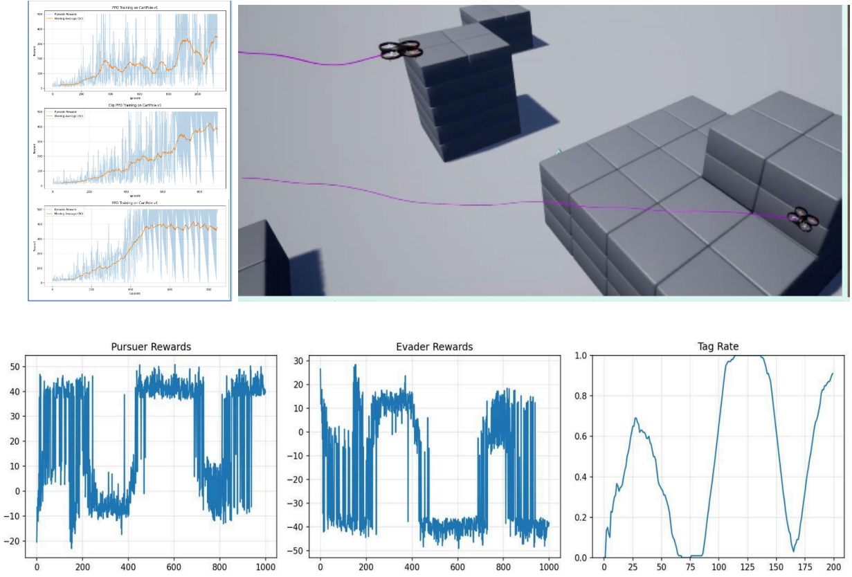
Figure 7. Self-play training curves. Left: per-episode pursuer reward over 1,000 episodes, showing oscillation between training phases. Center: evader reward over the same window, mirror-symmetric in expectation. Right: average tag rate over evaluation episodes per round. The dip mid-training corresponds to the introduction of the obstacle and the evader-speed increase; the tracker recovers to a final tag rate of approximately 0.95.
