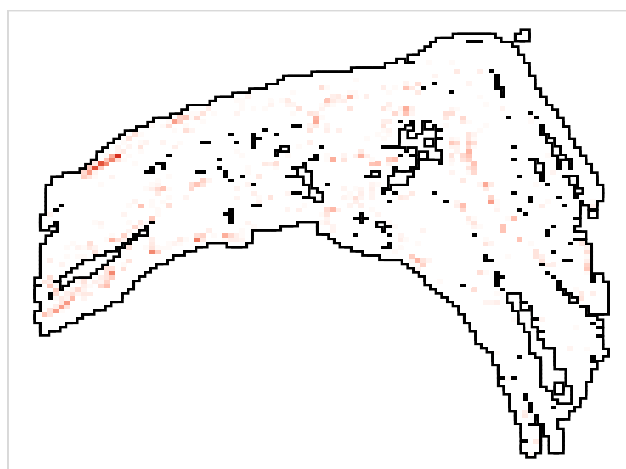
Stromal cells (DN) (n = 2,916)
