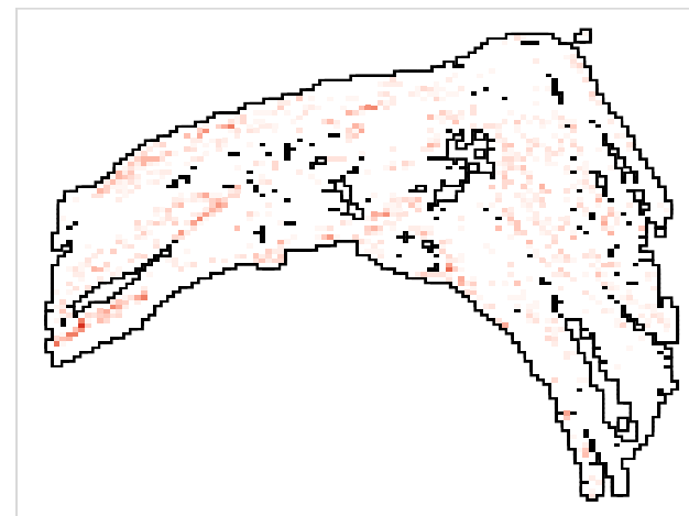
Endothelial cells (n = 3,727)
