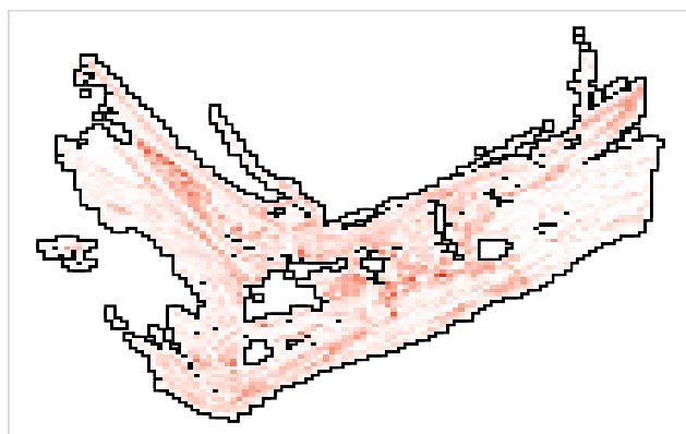
Fibroblasts (n = 31,846)
