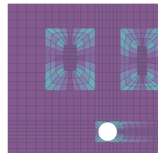
TOP-DOWN MESH
