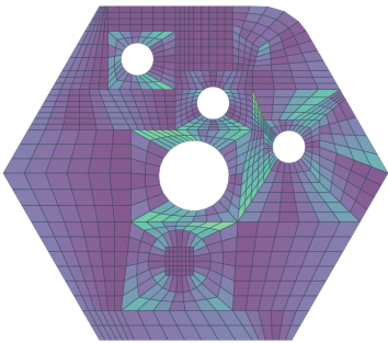
TOP-DOWN MESH
