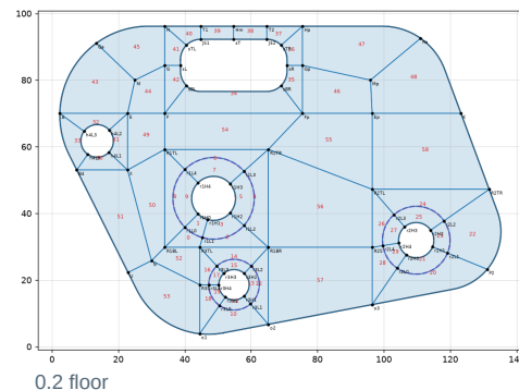
BLOCK LAYOUT
