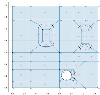
BLOCK LAYOUT
