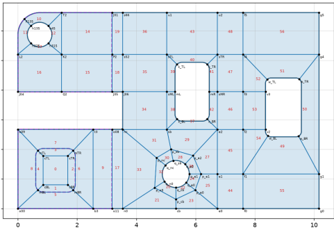
BLOCK LAYOUT
