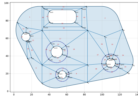
BLOCK LAYOUT
