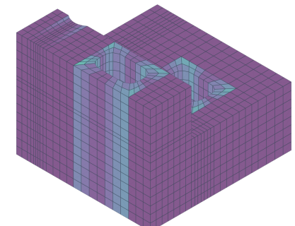
ISOMETRIC MESH
