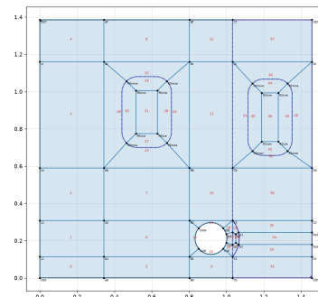
BLOCK LAYOUT
