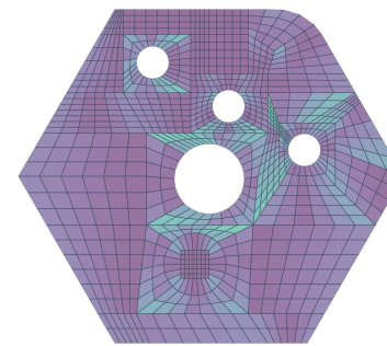
TOP-DOWN MESH
