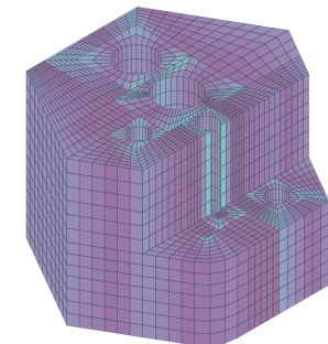
ISOMETRIC MESH
