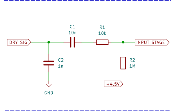
Input Stage
