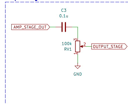
Output Stage
