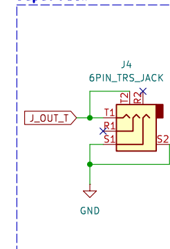
Ouput Jack
