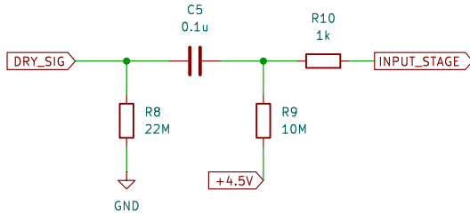
Input Stage
