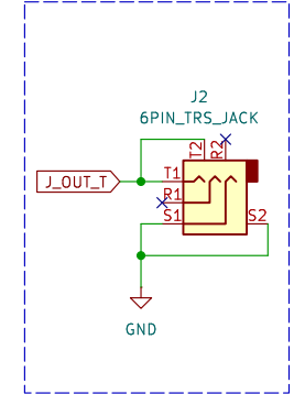
Output Jack
