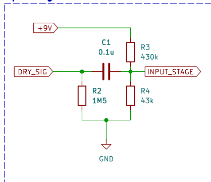
Input Stage
