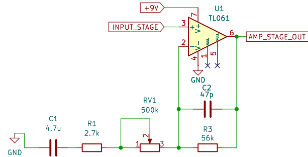
Amplifier Stage
