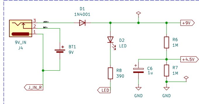
Power Circuitry
