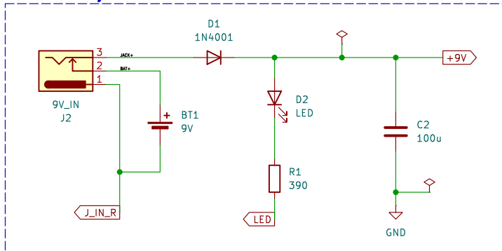
Power Circuitry
