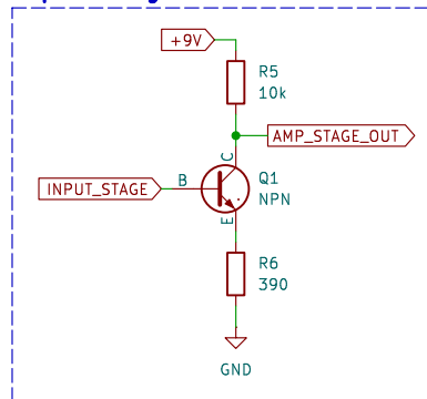
Amplifier Stage
