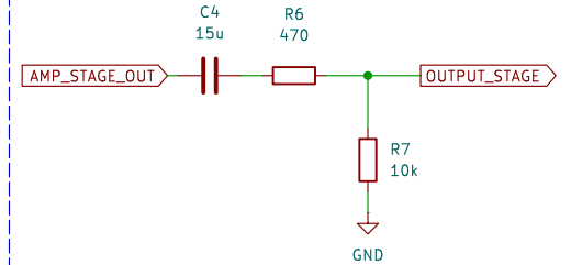
Output Stage
