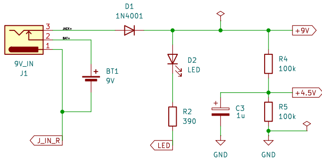
Power Circuitry
