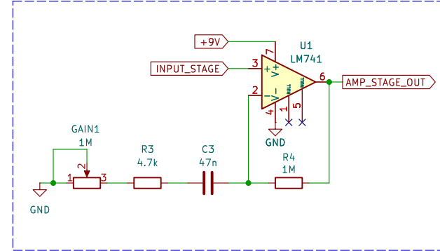
Amplifier Stage
