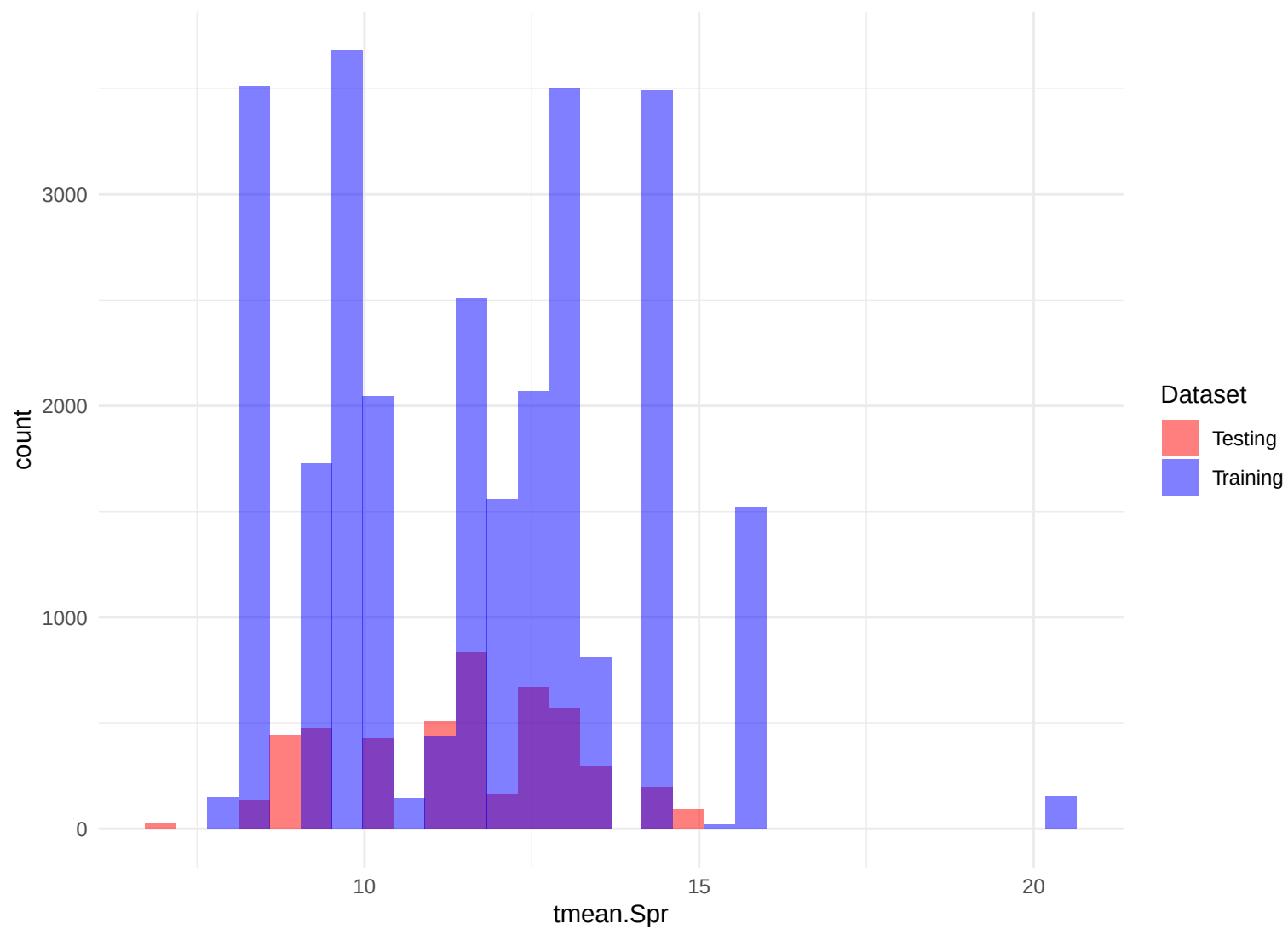
Histogram of tmean.Spr
