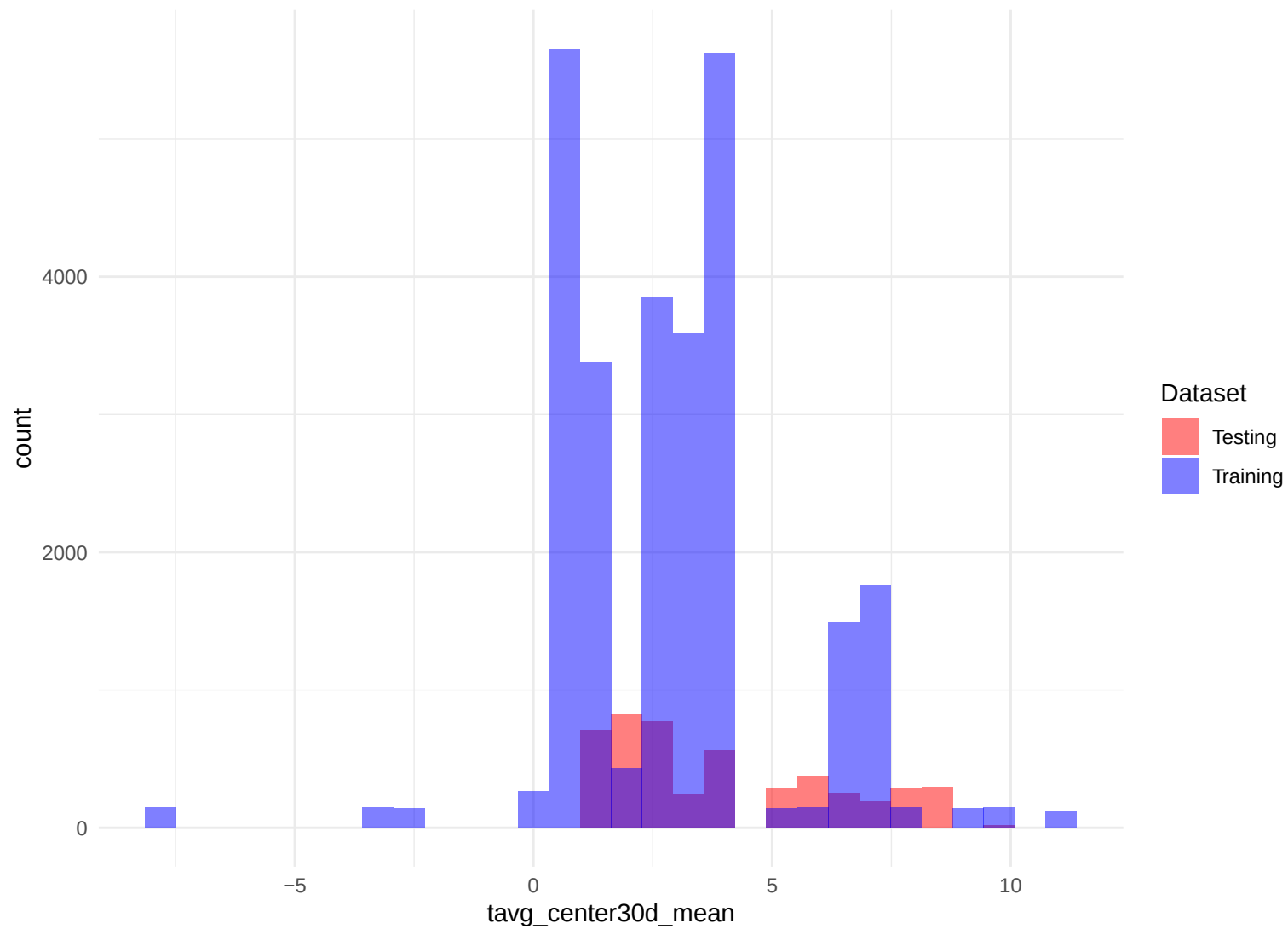
Histogram of tavg_center30d_mean
