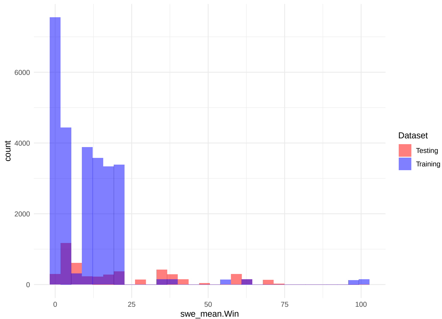
Histogram of swe_mean.Win
