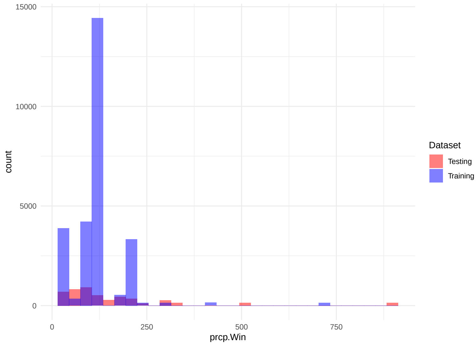
Histogram of prcp.Win
