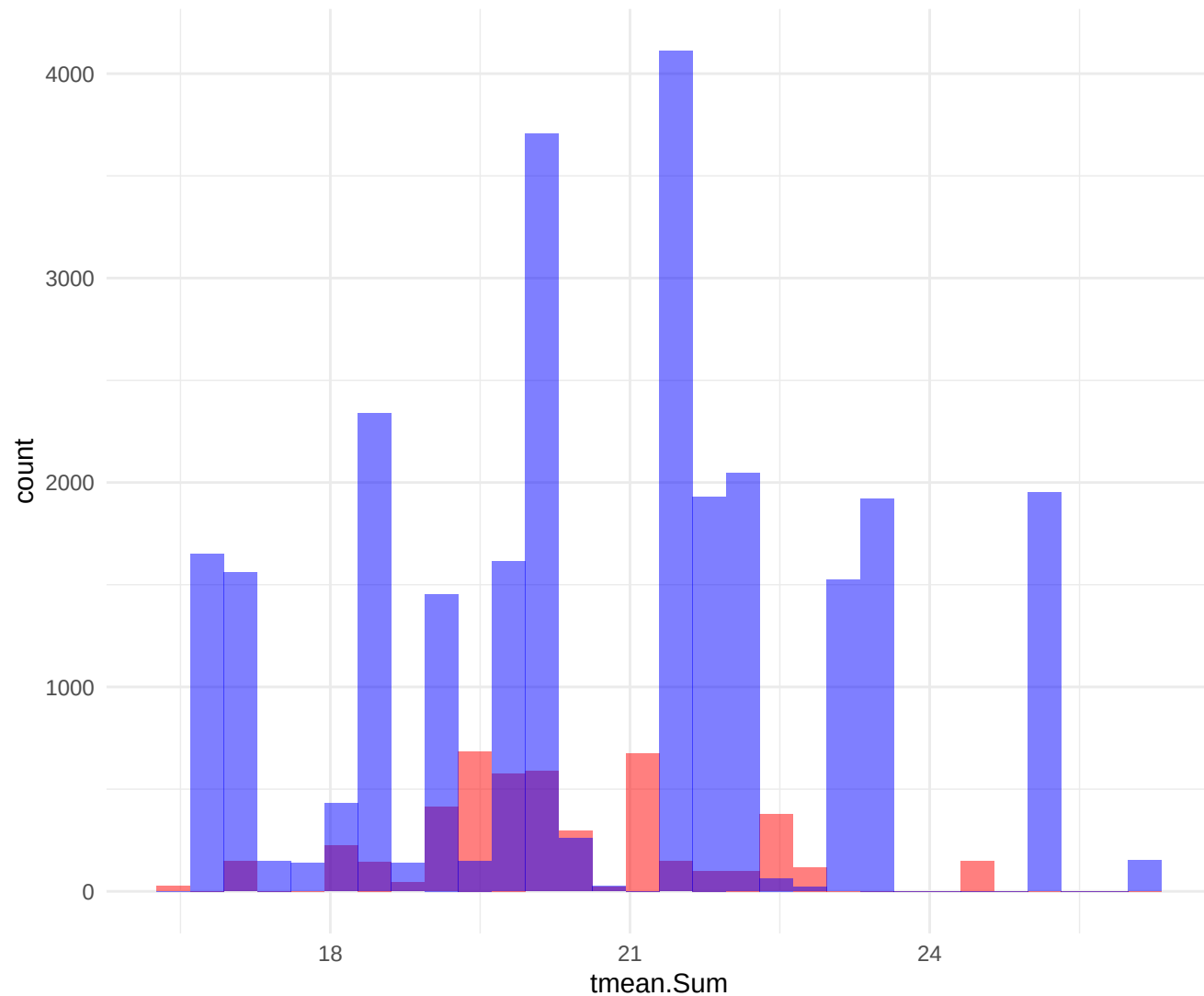
Histogram of tmean.Sum
