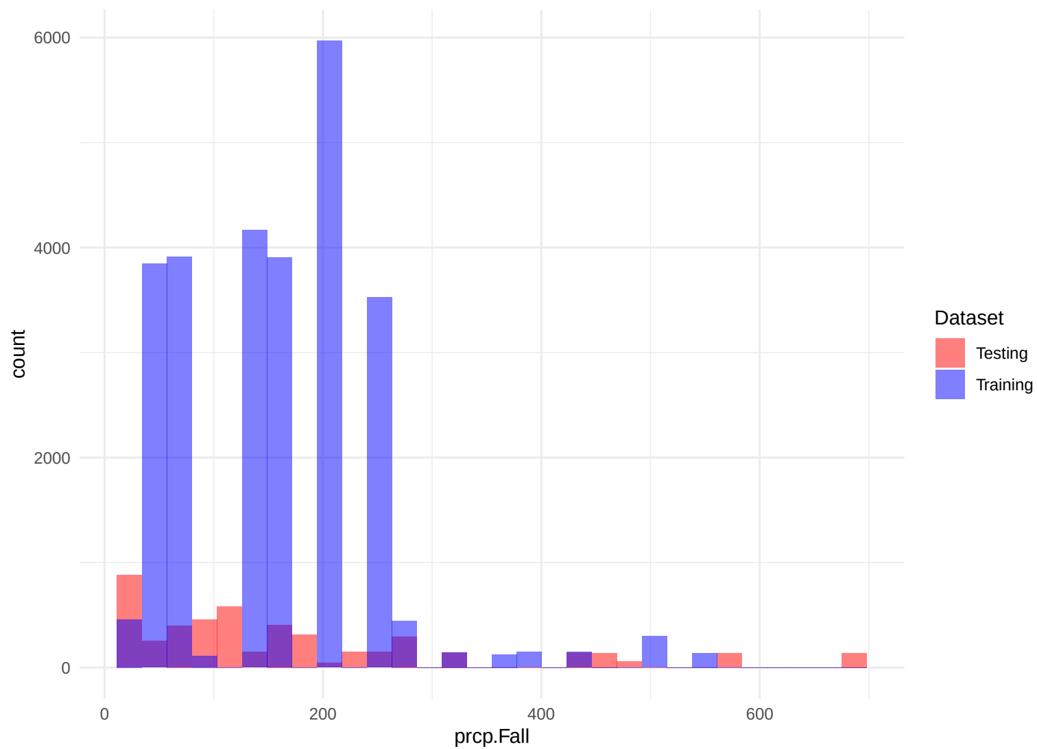
Histogram of prcp.Fall
