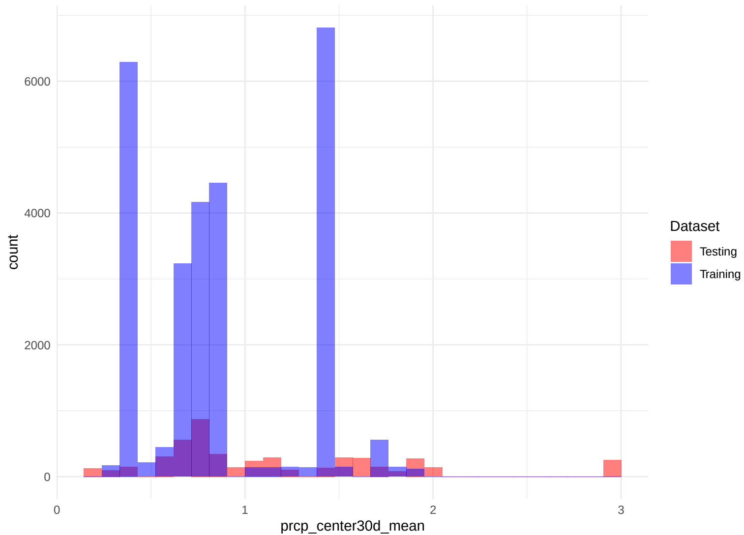
Histogram of prcp_center30d_mean
