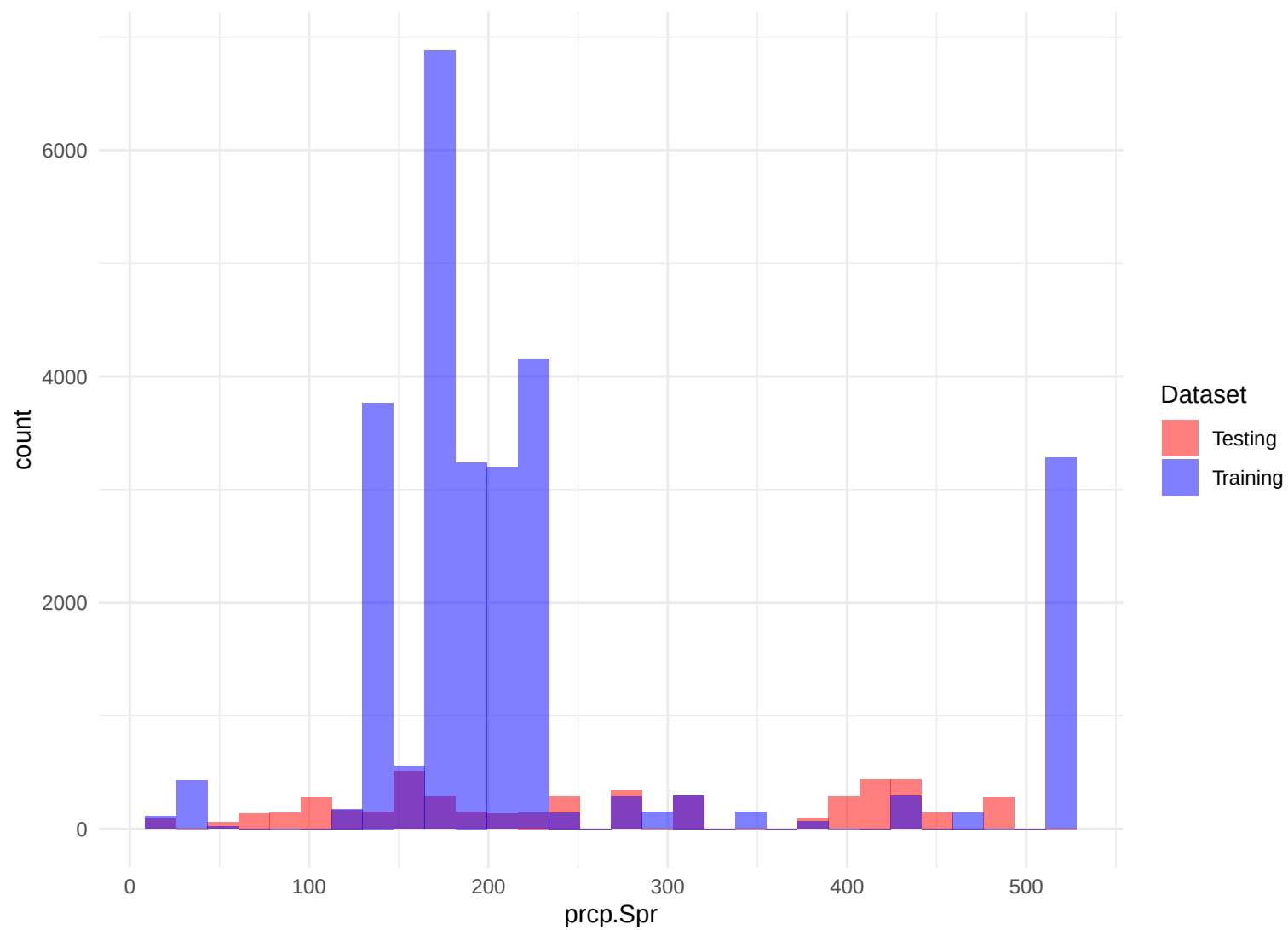
Histogram of prcp.Spr
