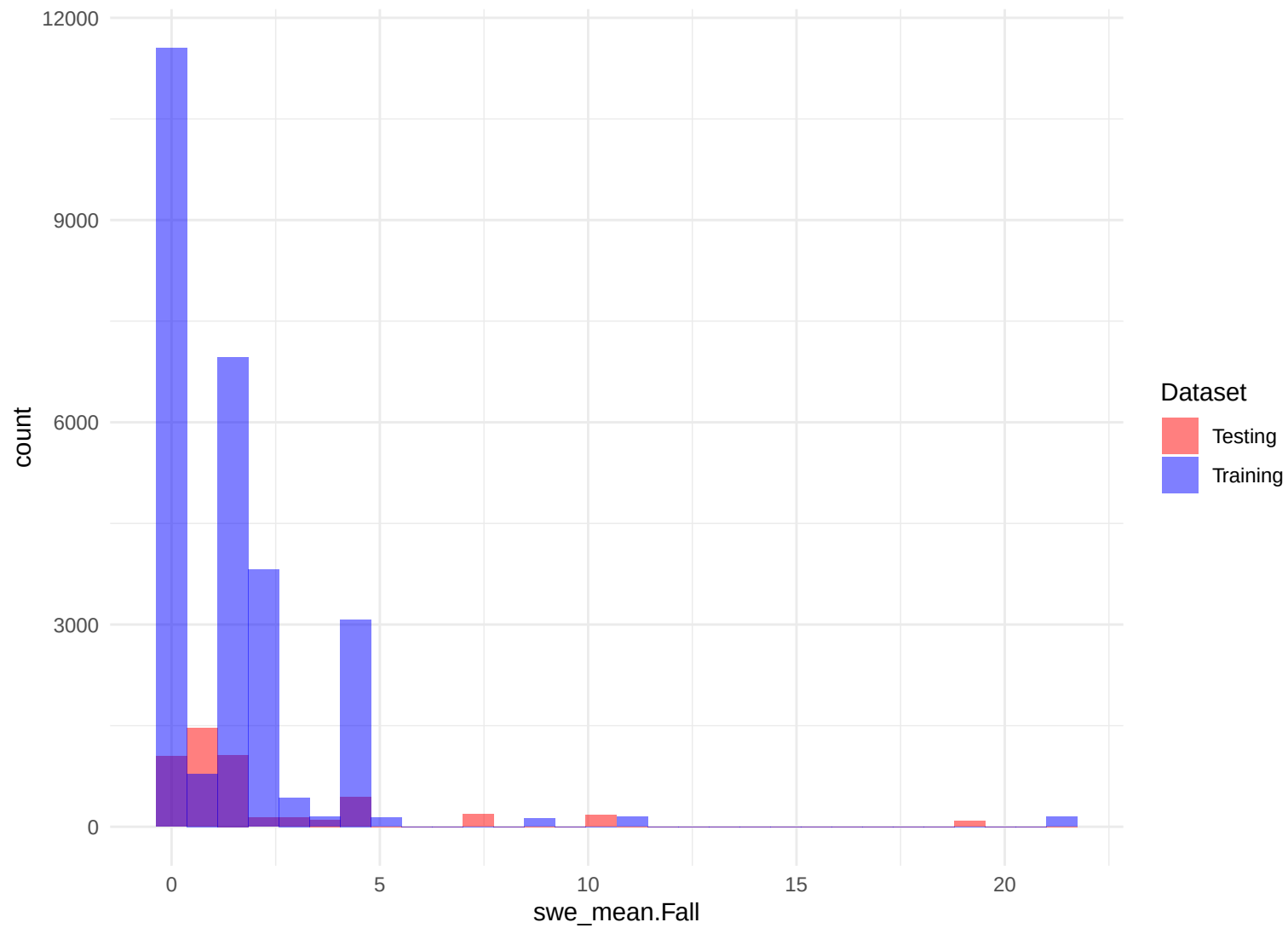
Histogram of swe_mean.Fall
