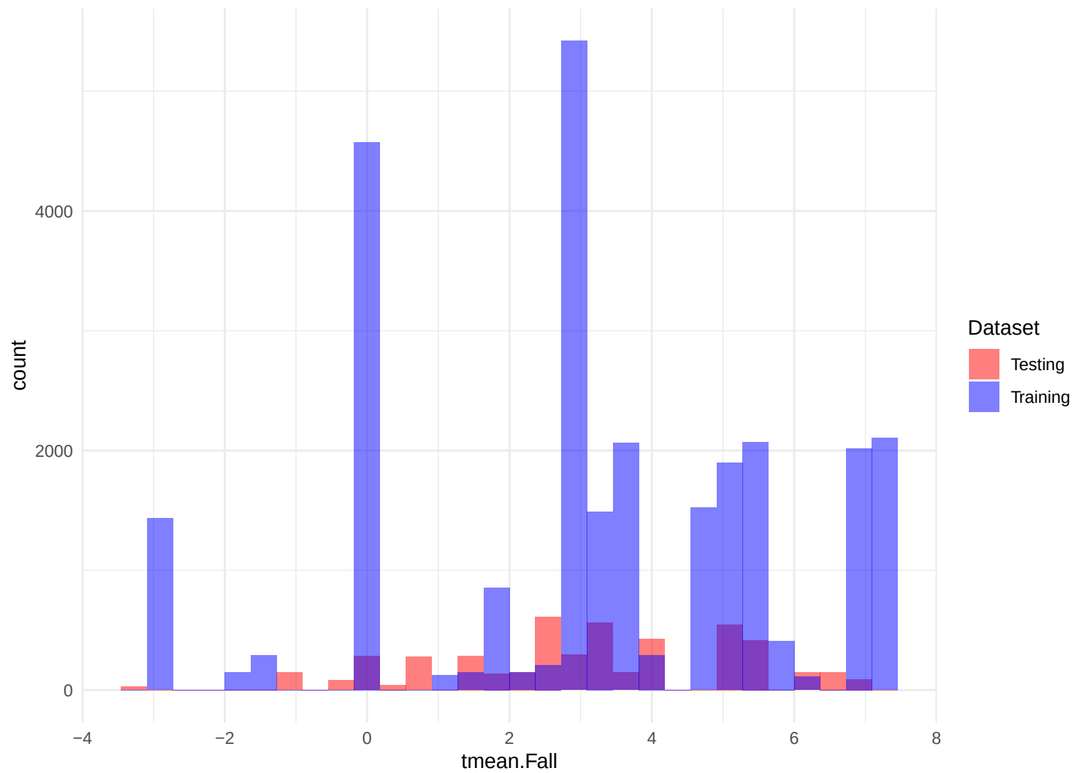
Histogram of tmean.Fall
