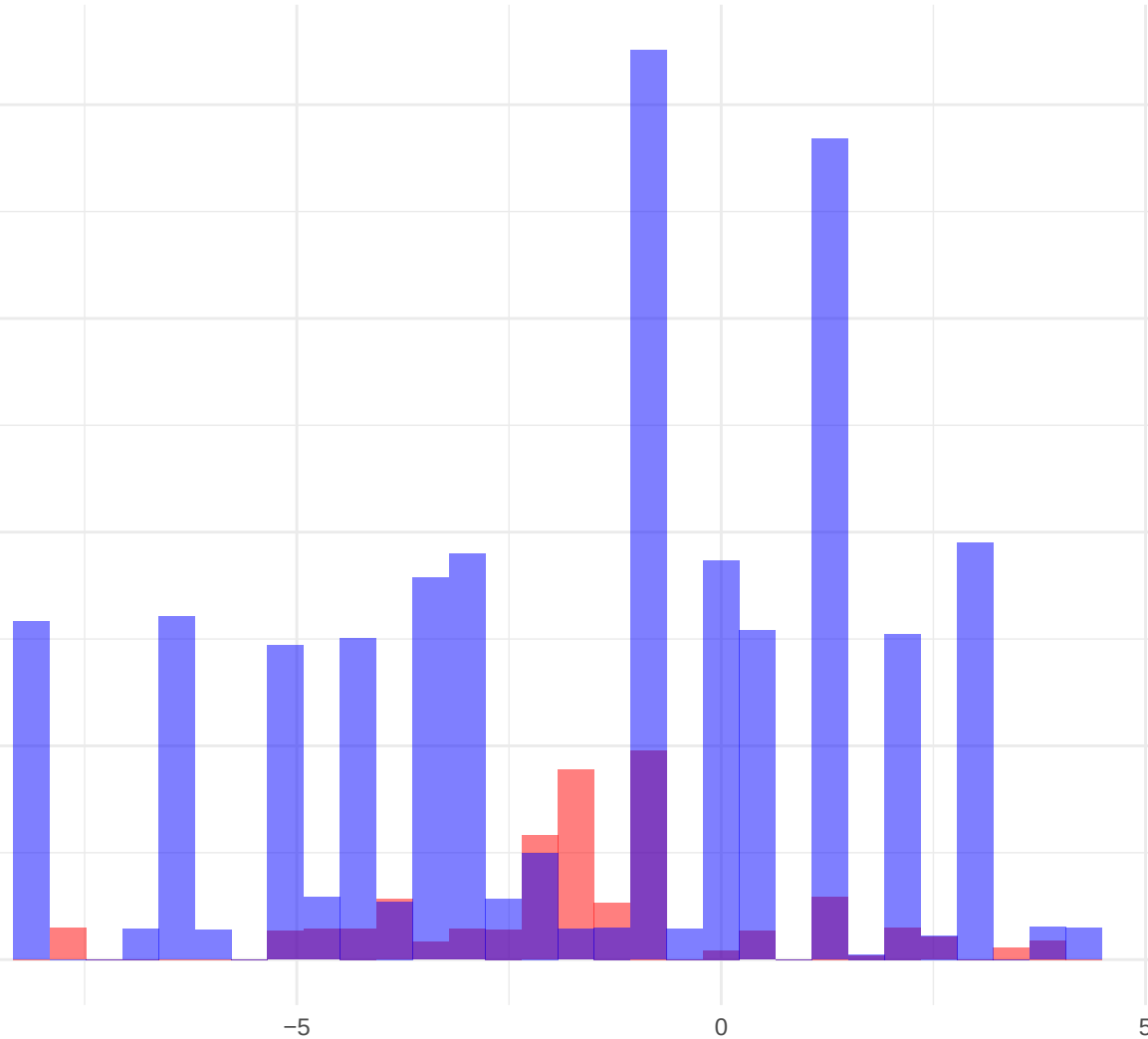
Histogram of tmean.Win
