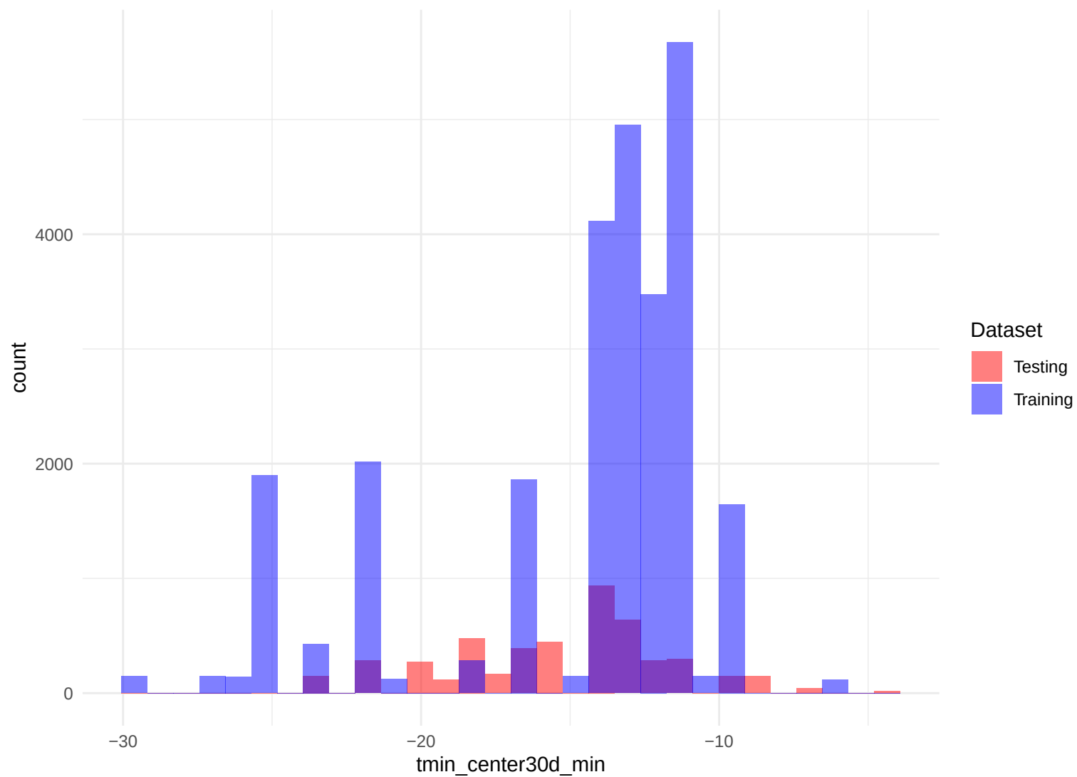
Histogram of tmin_center30d_min
