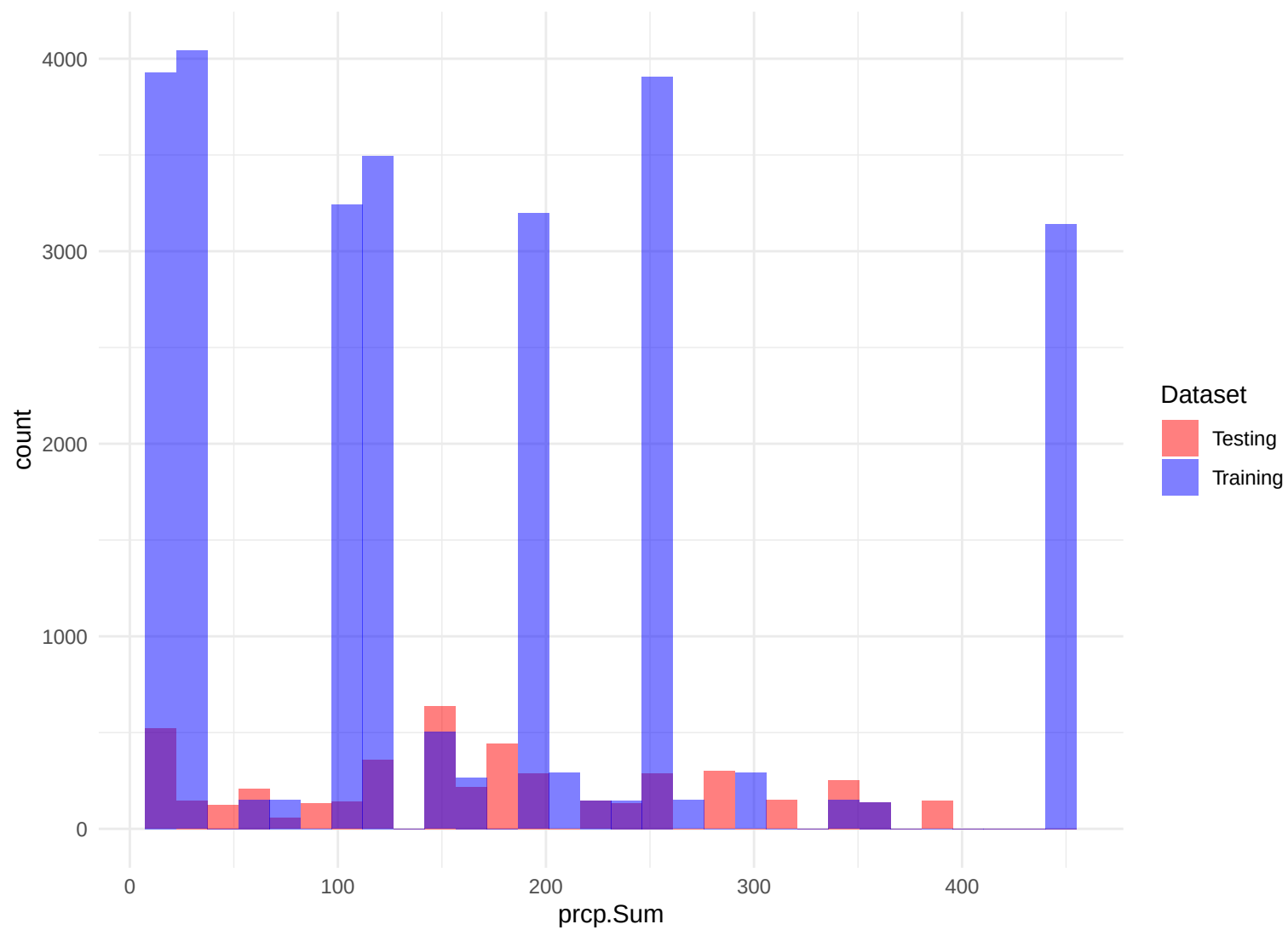
Histogram of prcp.Sum
