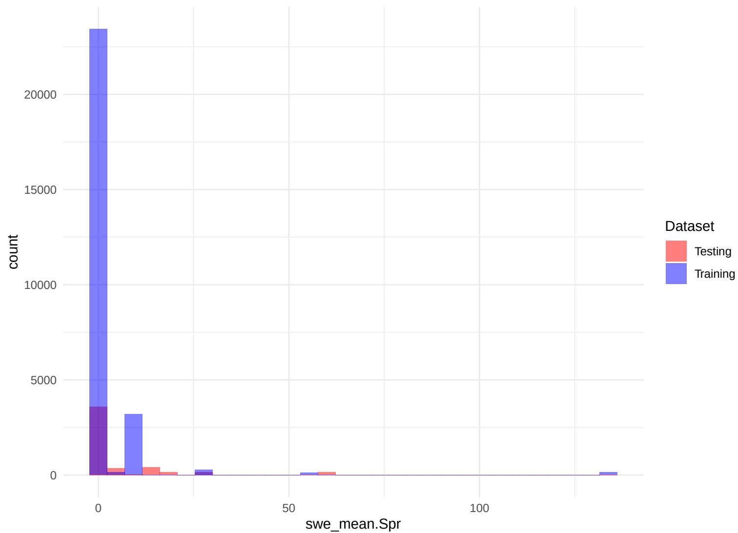
Histogram of swe_mean.Spr
