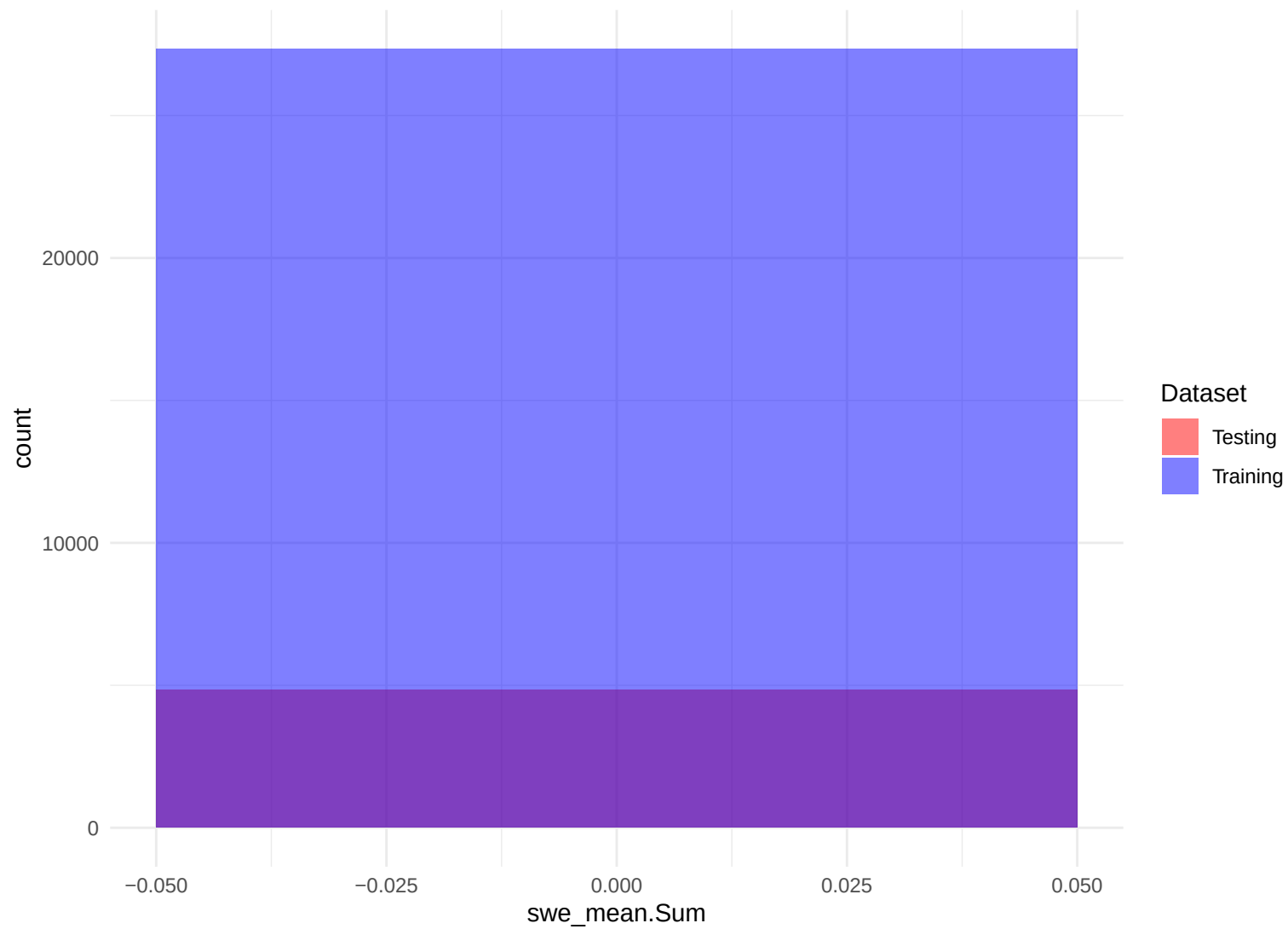
Histogram of swe_mean.Sum
