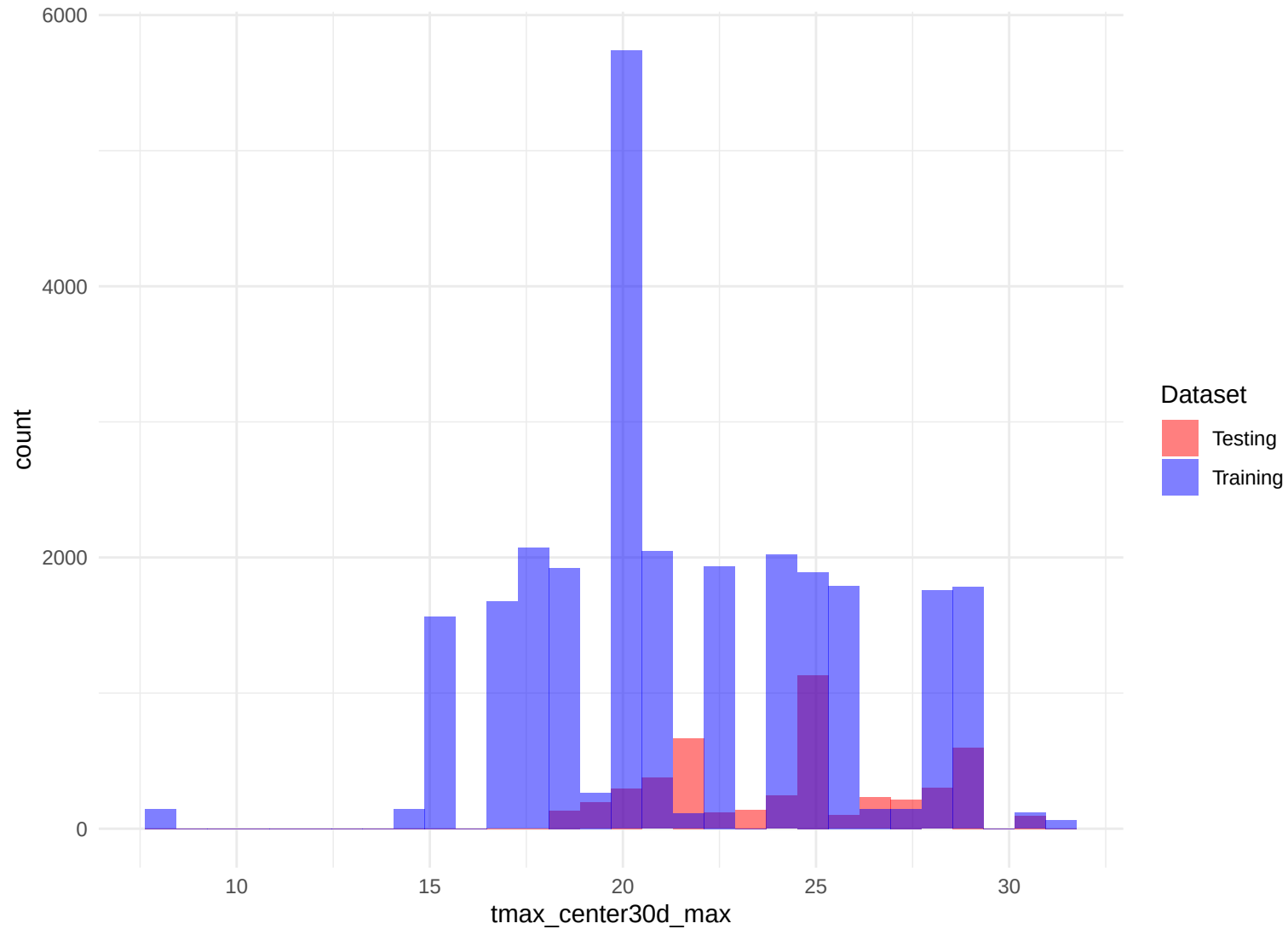
Histogram of tmax_center30d_max
