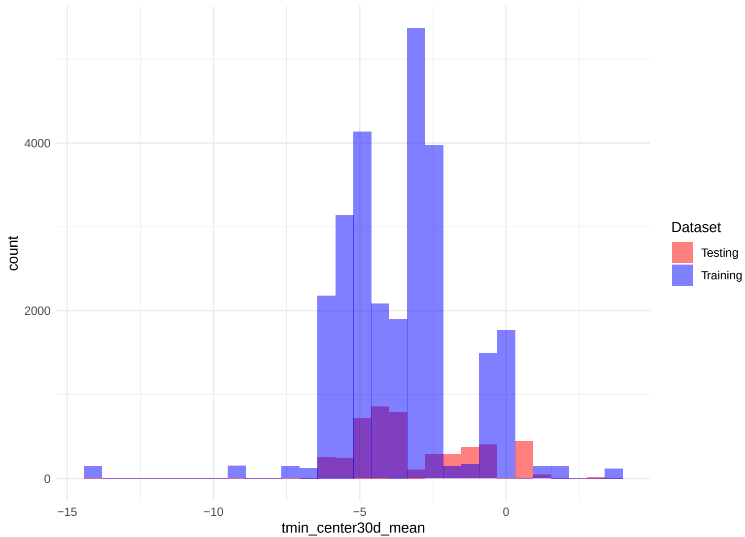
Histogram of tmin_center30d_mean
