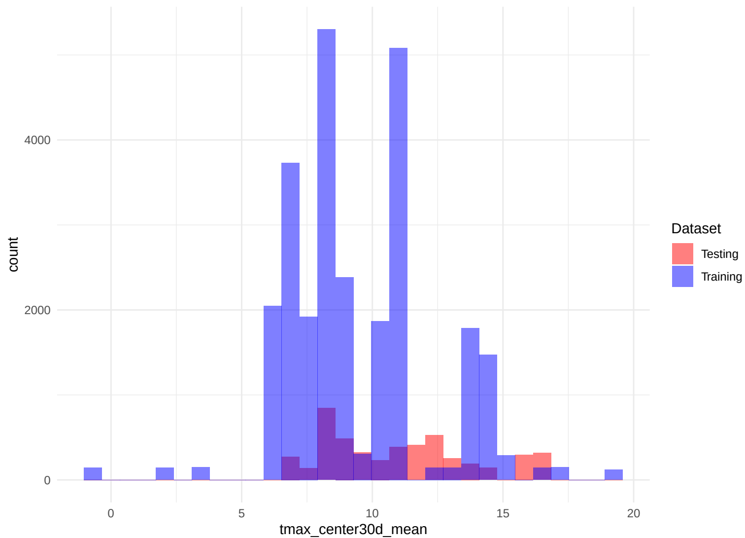
Histogram of tmax_center30d_mean
