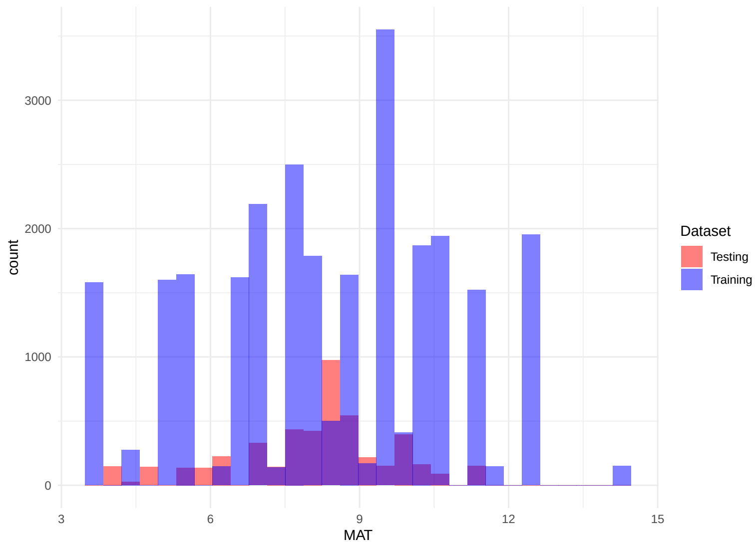
Histogram of MAT
