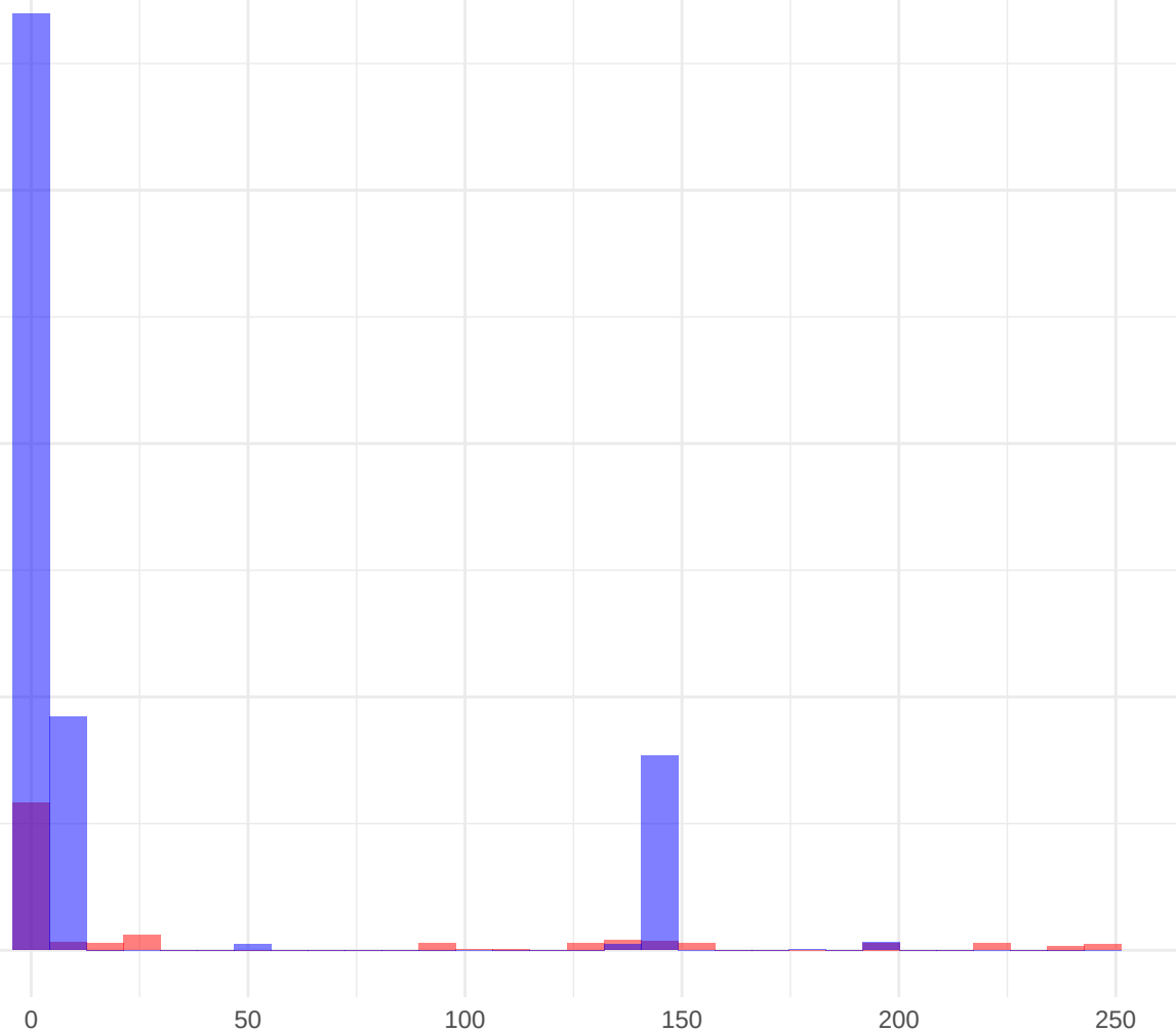
Histogram of seasonality
