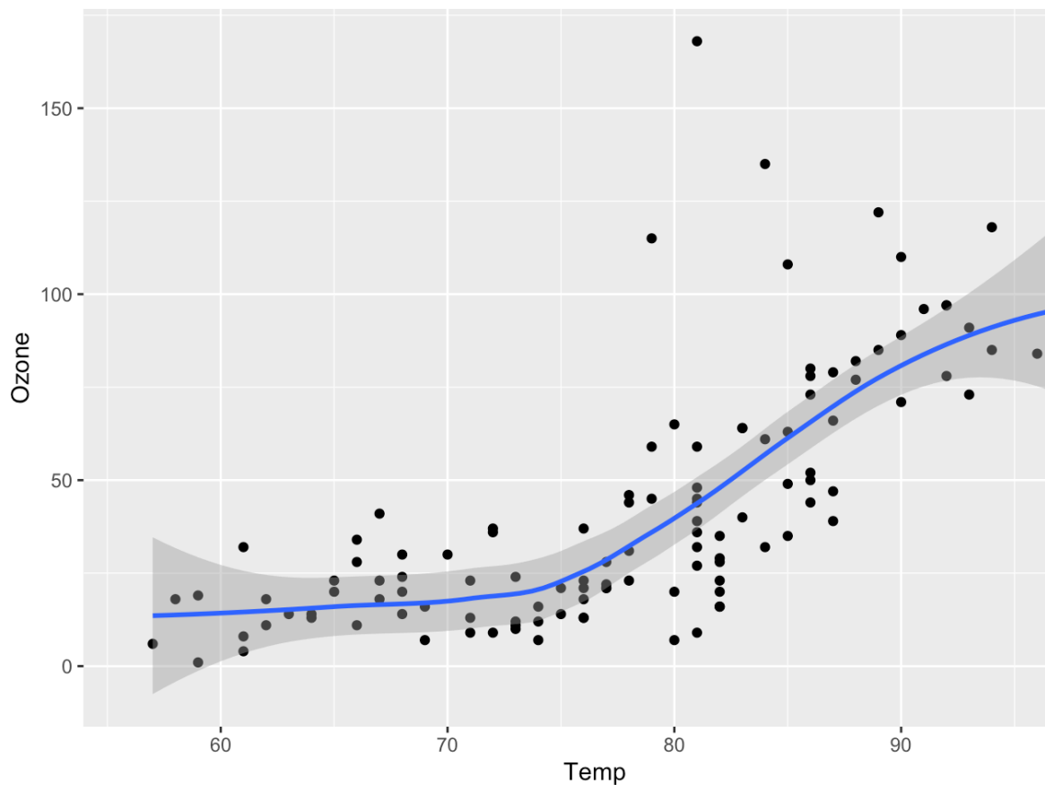
Figure 1: Temperature and ozone level.
