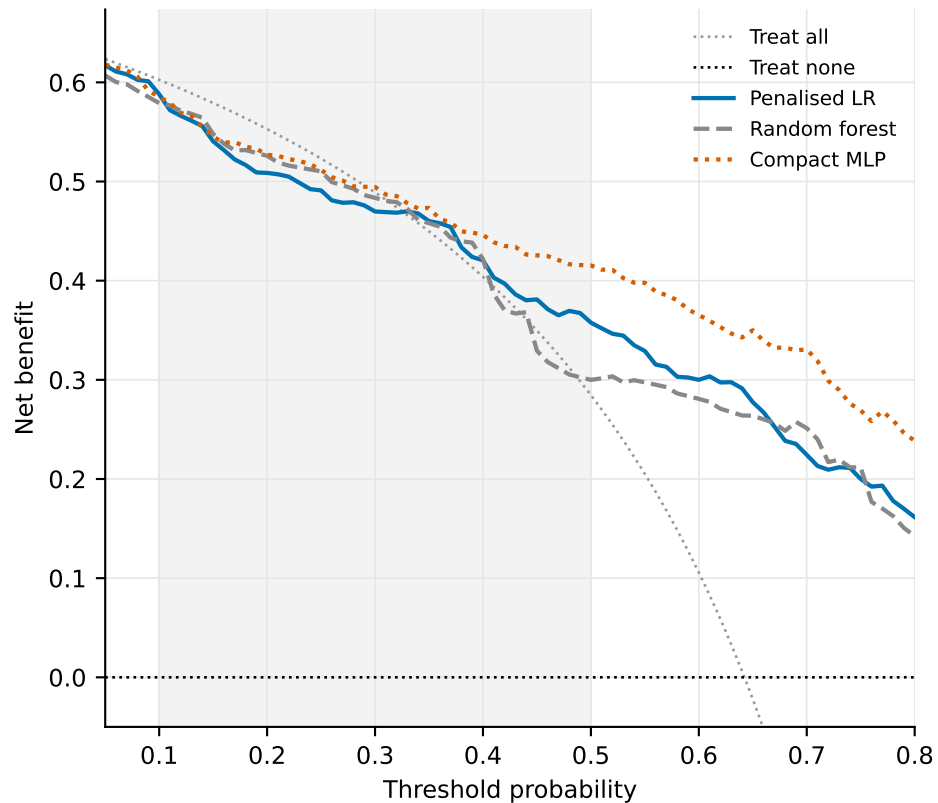
Decision-curve analysis — Gravendeel (external)
