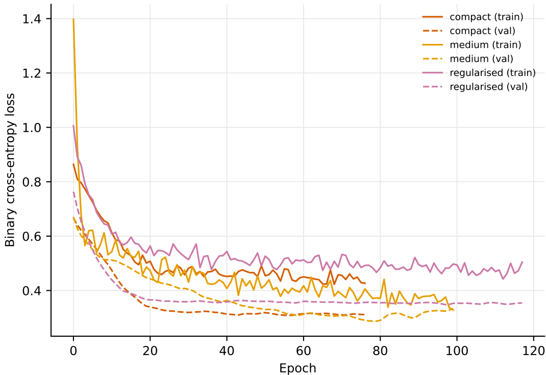
Neural-network training and validation loss (TCGA, set B)
