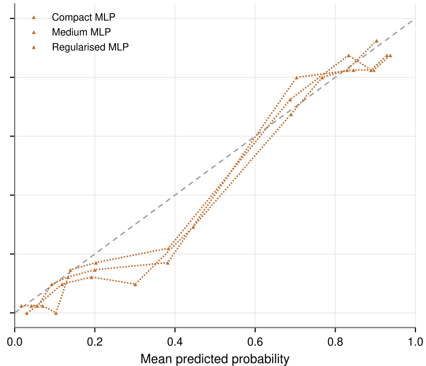
Neural networks
